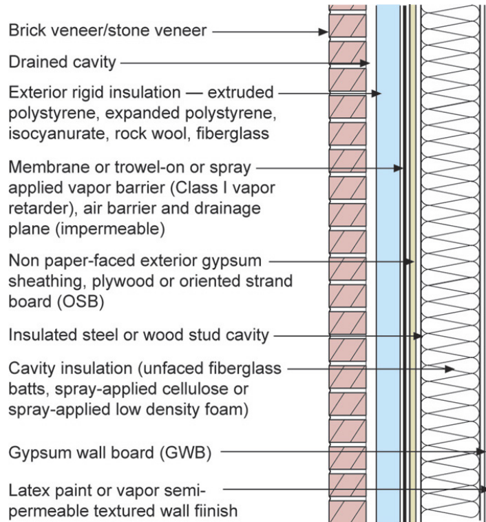
Figure 8 Frame Wall With Exterior Rigid Insulation With Cavity Insulation and Brick or Stone Veneer
