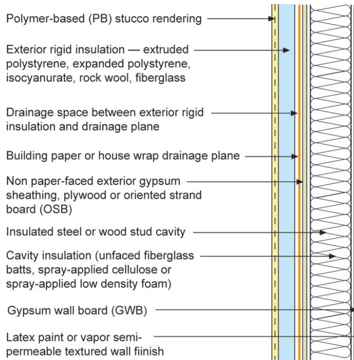
Figure 13 Frame Wall With Exterior Rigid Insulation With Cavity Insulation and Stucco
