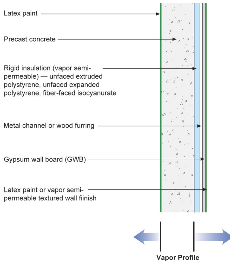
Figure 15 Precast Concrete With Interior Rigid Insulation
