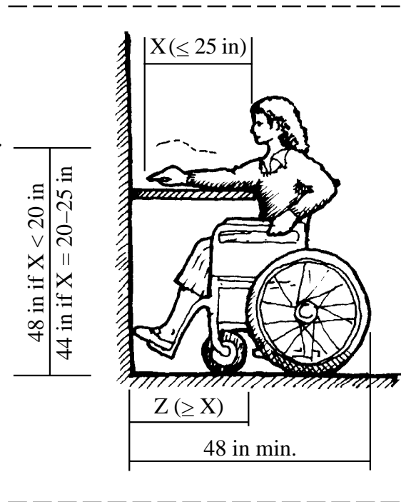
Figure 2-6: Maximum forward-reach over an obstruction (PLAE, Inc., 1993).
