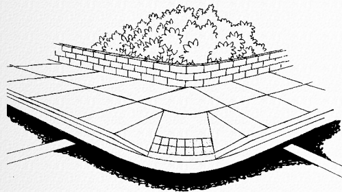
Figure 7-5. When designed to promote access, diagonal curb ramps include a detectable warning, a clear space of at least 1.220 m (48 in) within the crosswalk, and a level maneuvering area at the street/gutter approach.
