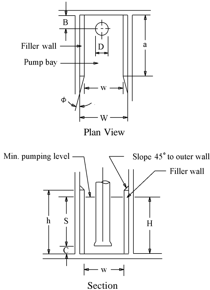
Figure 9-2. Filler walls for pump bay Adapted from reference 15
