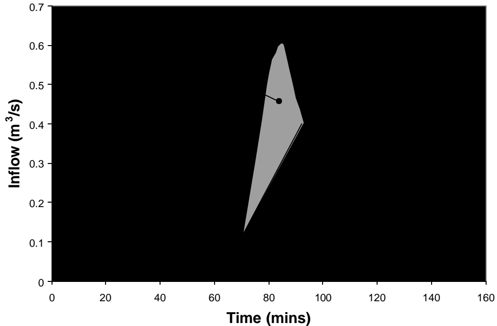
Figure 6-3. Estimate of storage required
