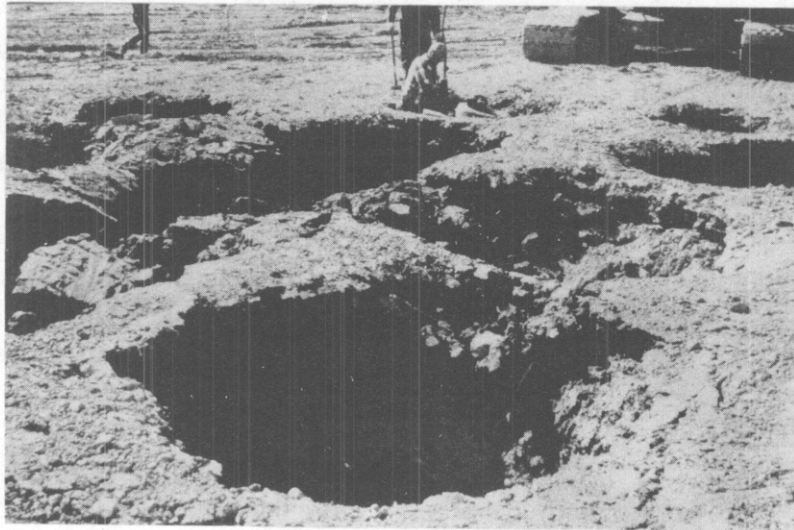
Figure 23. Ground heave induced by dynamic compaction.
