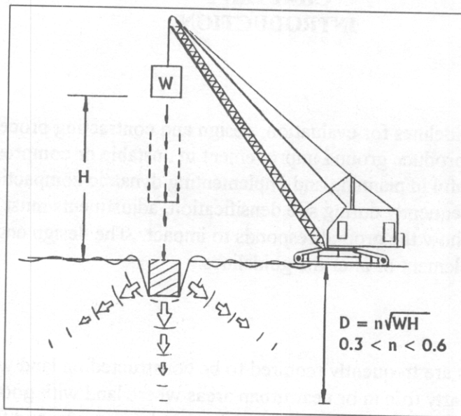
Figure 1. Dynamic compaction.
