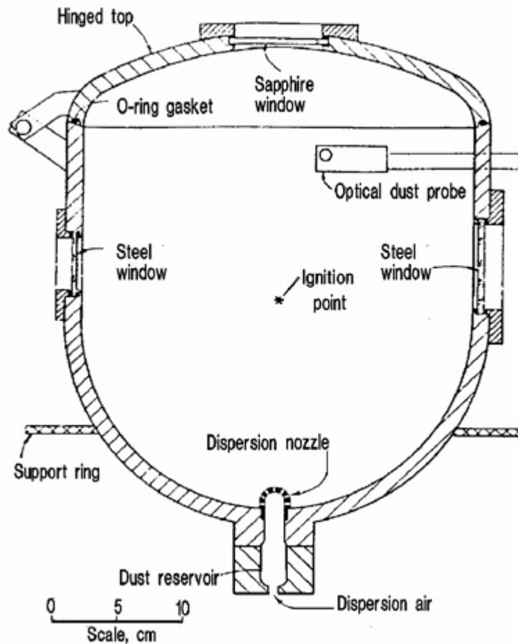
Figure 1: 20-Liter Explosibility Test Chamber
