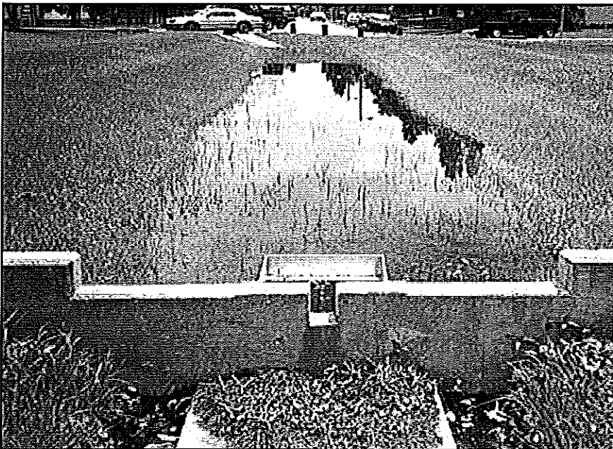
▲ Outlet Structure.
