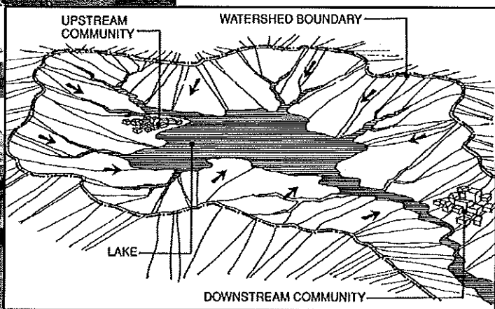
▲ A watershed is the land that water flows across or under on its way to a stream, river or lake.
