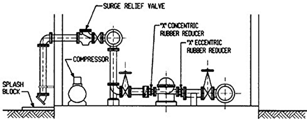
A SECTION
