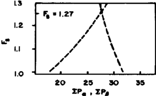
Figure 7 (continued) Example of Stability Analysis of Translational Failure
