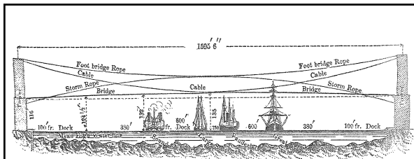
Bridge Cable Diagram
