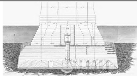
Transverse Section through the Brooklyn Caisson Offering a good front elevation and sectional view of a frame (with its two openings and diagonal cladding). Also in view are the masonry courses atop the caisson (always several feet above the waterline). It also provides a good sectional view of the roof structure and one (of two) air-lock/s and shaft/s (w/ladder) and the "pool" below a water shaft (water shaft/s not in view).
