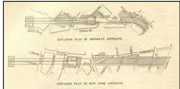
Plan of Brooklyn (top) and NY (bottom) approach (note the increased length and multiple intersecting streets for the NY Approach as compared to the Brooklyn Approach) 458
