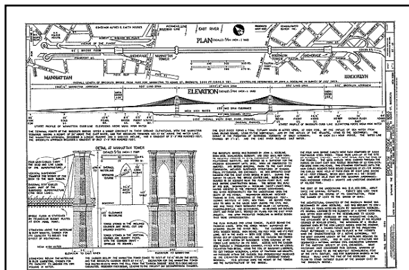
General Plan & Elevations by JAR
