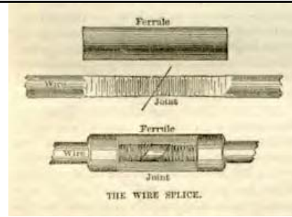
The Ferrule (wire splice)
