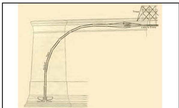
Longitudinal cross-section through anchorage Showing anchor chain base plate/s and double row of arc-shaped eye-bar chain/s secured to end/s of cable/s 341
