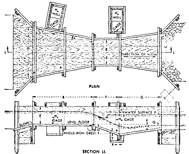
Courtesy of Fairbanks Morse, Inc., Pump Division Figure F-11. Plan and elevation of the Parshall measuring flume.
