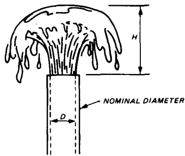
U. S. Army Corps of Engineers Figure F-8. Fountain flow measurement.
