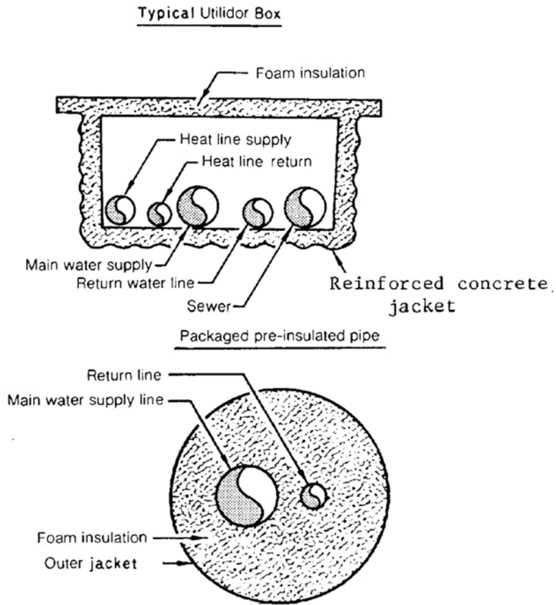
Figure 2 Typical utilidor and packaged preinsulated pipe
