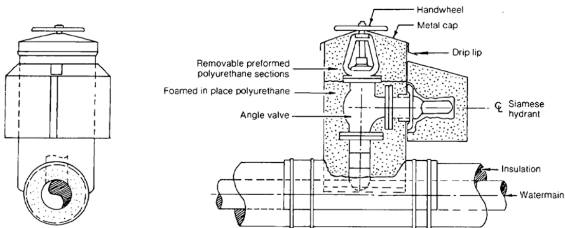
Figure 9 Above-ground hydrant
