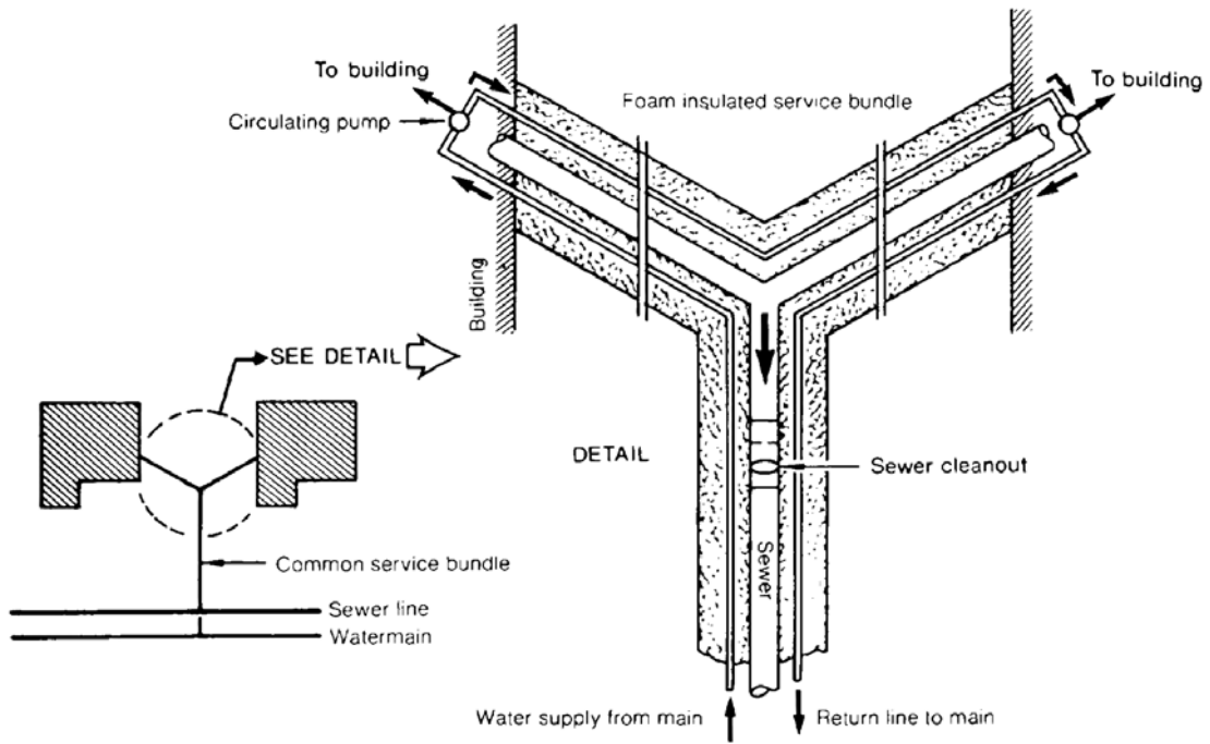
Figure 8 Dual service
