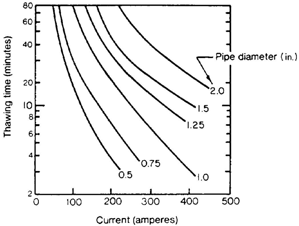
Figure 13 Approximate times and current for thawing steel pipes
