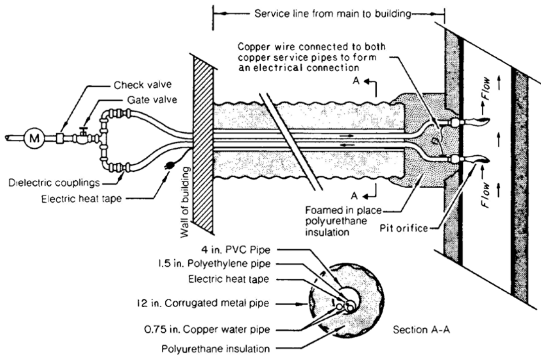
Figure 4 Water service line, with pit orifices
