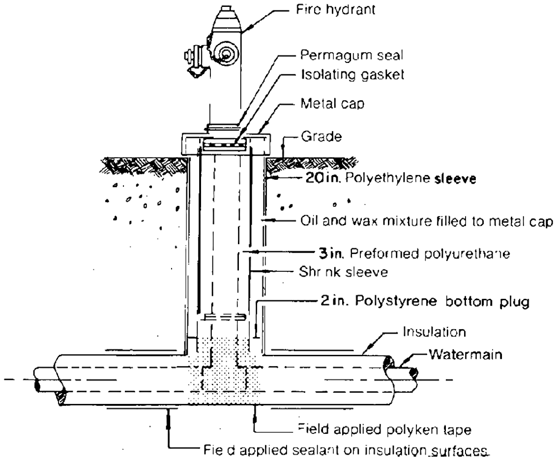
Figure 10 Below-ground hydrant
