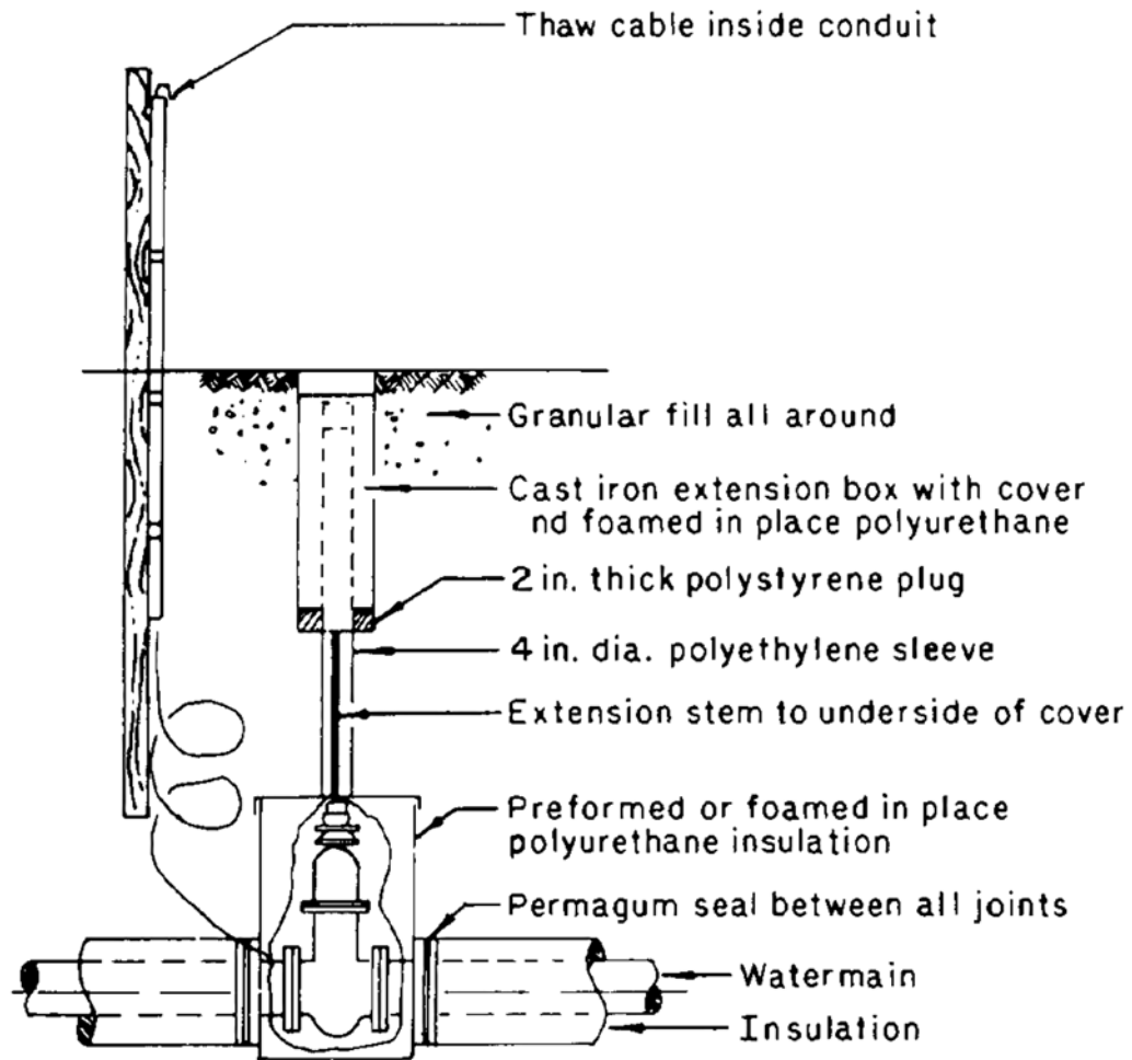
Figure 7 Underground valve and box
