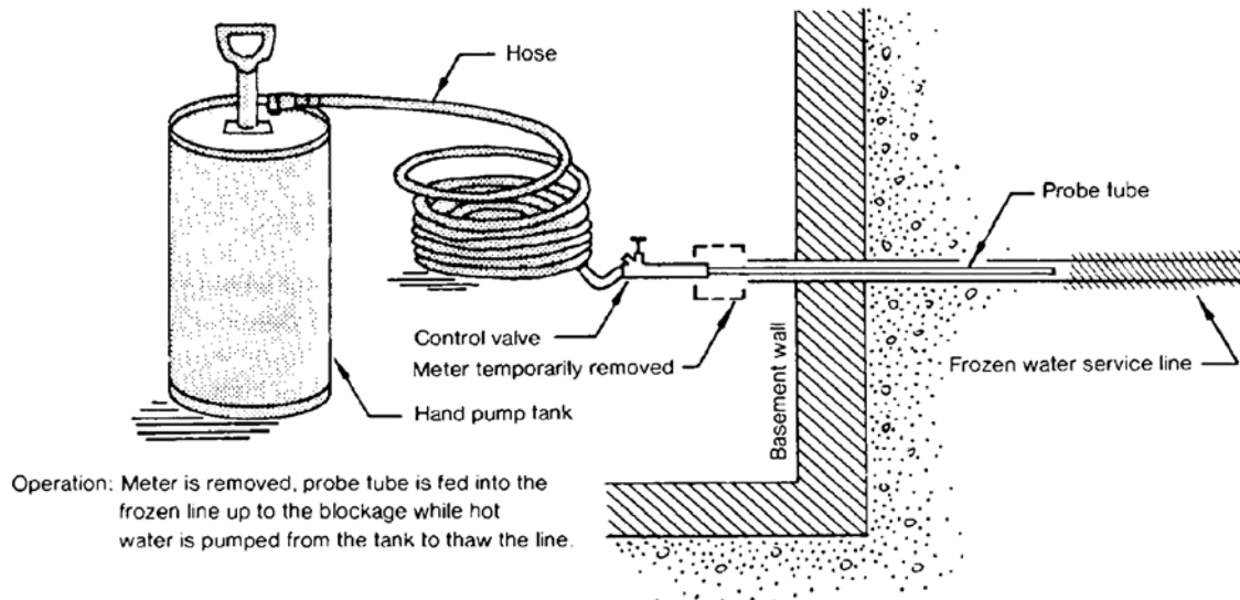
Figure 11 Thaw tube, thawing method
