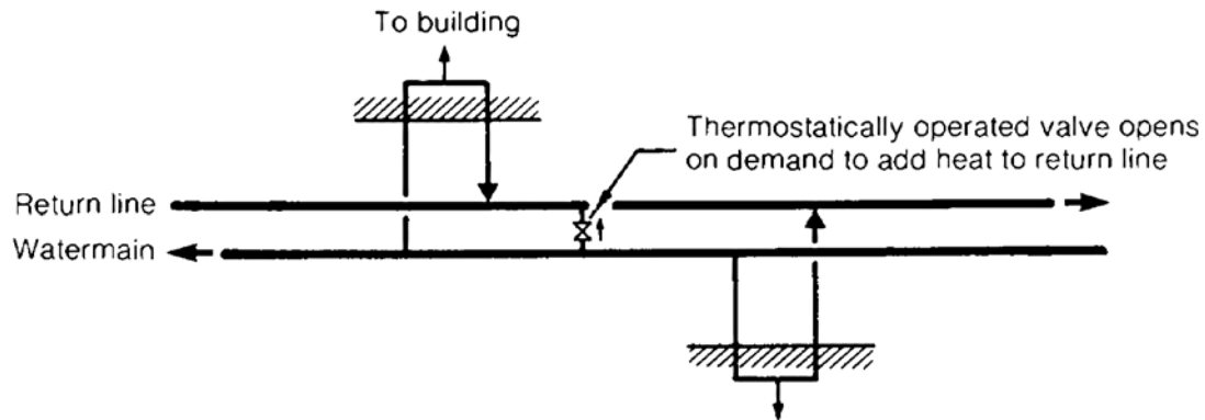
Figure 3 Schematic diagram of a dual pipe system
