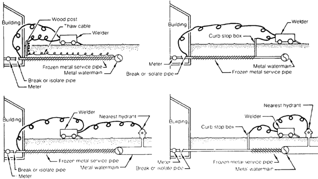
Figure 12 Alternatives for thawing service lines
