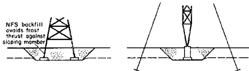
c. Gravel backfill with buried footings
