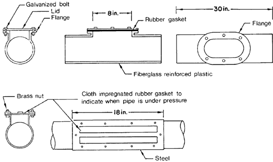
Figure 1-5 Sewer cleanouts
