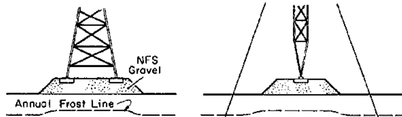
Trussed Tower Guyed Tower a. Gravel mat with surface footings
