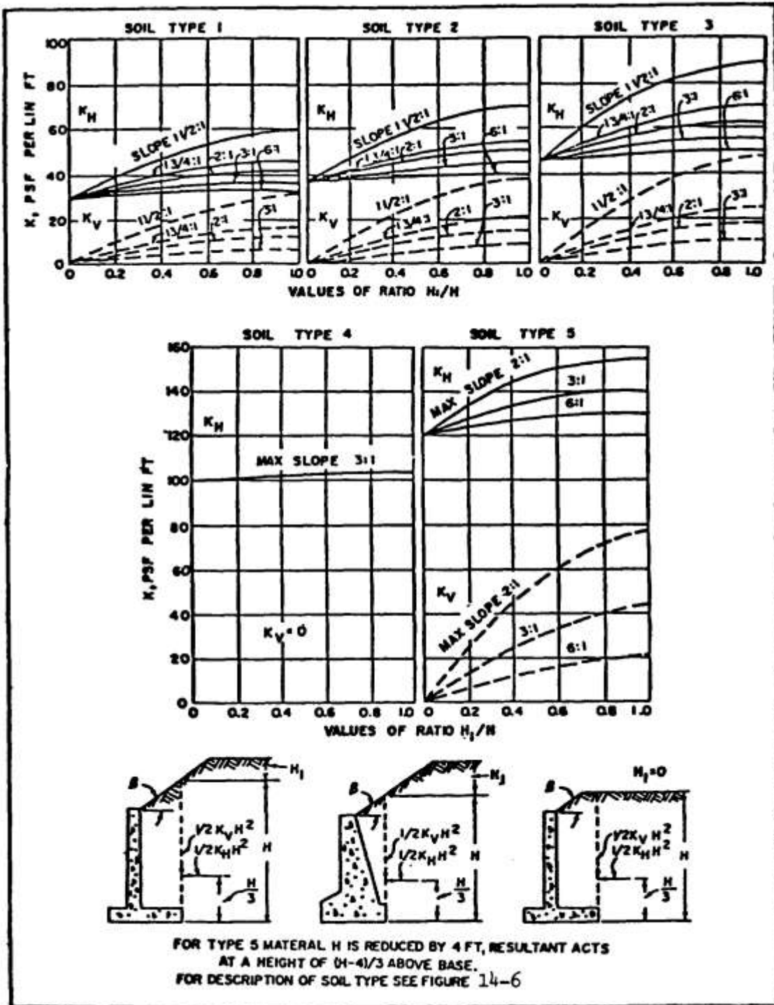
Figure 7 Design loads for low retaining walls, broken slope backfill
