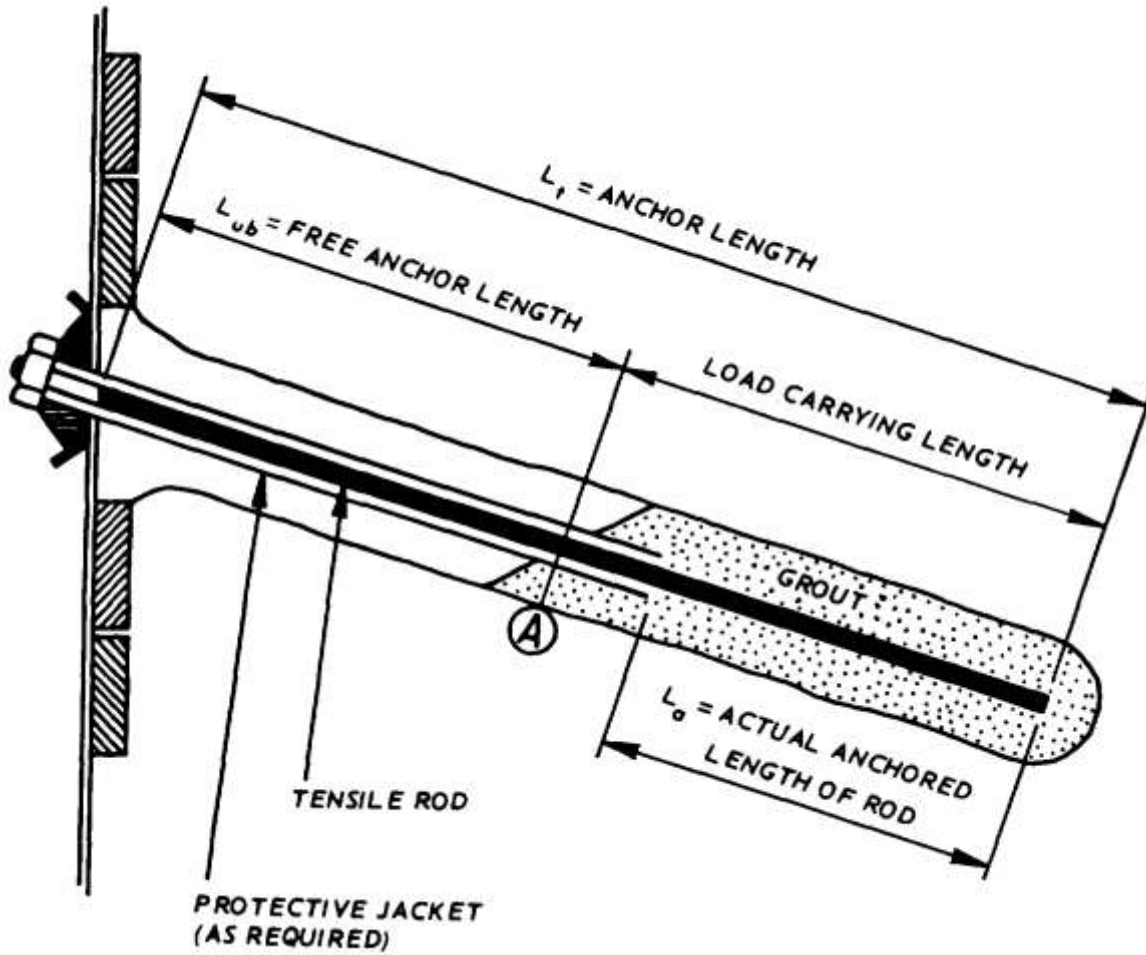
Figure 13 Typical tieback details
