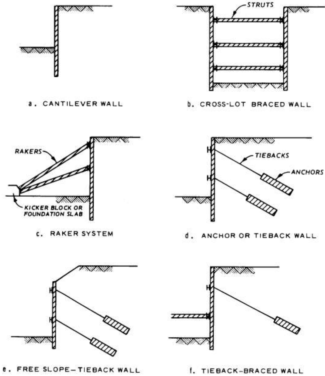
Figure 10 Types of support systems for excavations
