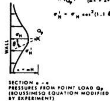
Figure 5 Horizontal pressures on walls due to surcharge
