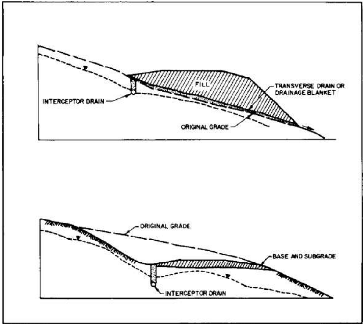
FIGURE 8 Intercepting Drains for Roadways on a Slope
