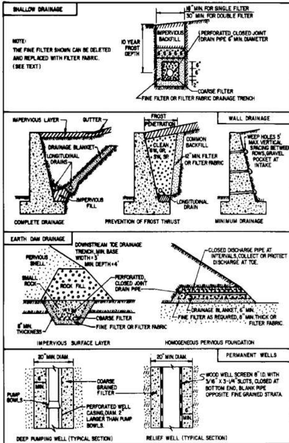
FIGURE 5 Typical Filter and Drainage Blanket Applications
