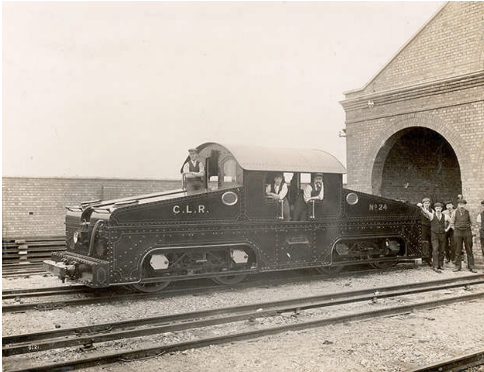
Above: an early underground electric train of the CLR. This engine could be driven in both directions.
