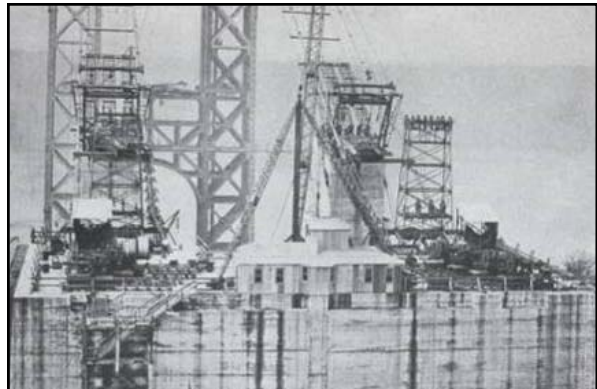
Above: caption: "Cable spinning equipment on New York anchor block. Traveling cages erecting north and south side span footbridges simultaneously." 322
