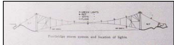
“...The footbridge storm system cables were assembled immediately below, and supported from the footbridges, and their connections were made from the footbridge erection travelers. The booms and ropes were lowered to position. The counterweights in the towers were attached, and the adjustments were made by men in bo'sn's chairs. The system reduces vertical and horizontal displacements from a 60-mile wind, to about 1 foot and 3 feet, respectively. It contains about 75,000 feet of 0.63, 1.75, and 2-inch rope. Besides providing an ample illumination with 200-watt lamps with domes, shades and reflectors for construction operations, the Roebling Co., maintains on the footbridge a complete system of all night traffic signal lights complying with United States and navigation requirements for aeroplane and marine traffic...”
