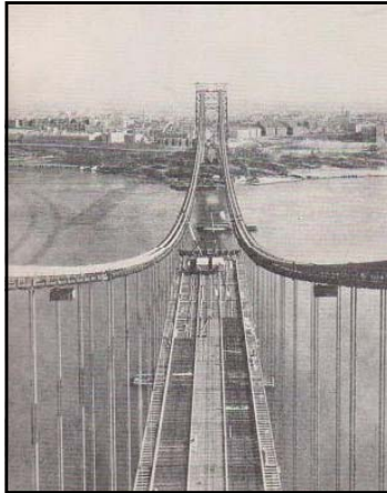
Left: caption: Building the Road Deck. Work proceeded simultaneously from either tower and the floor was completed on the central span in less than four months. This photograph was taken from the tower on the New Jersey side of the bridge.” Wonders of World Engineering, November 1937
