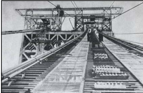
Above: caption: "Preparing upper end of center span footbridge for installation of electric signal system. Note Roebling construction tower on top of main tower in background." 355
