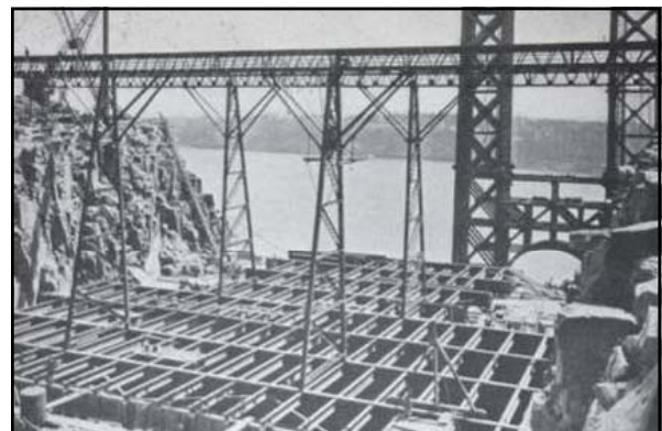
Above: caption: "New Jersey anchorage floor steel furnished and erected by the McClintock Marshall Co., under Roebling contract. Also crane runway for handling reels of bridge wire and equipment at the New Jersey anchorage." 258
