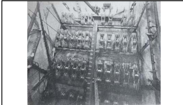
Above caption: "Lower panels of New Jersey anchorage eyebars for two main cables ready for successive connections with upper tier of eyebars that engage the strand shoes. Boom for handling equipment above. Pipes from hydraulic pumps, on the walls. Pressure tubes to strand pulling jacks at lower right corner."
