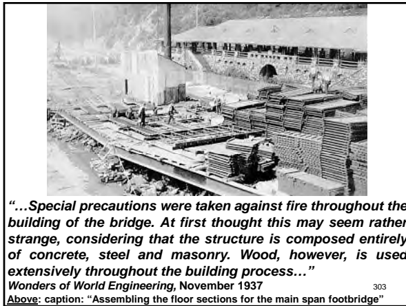
Above caption: “Assembling the floor sections for the main span footbridge”
