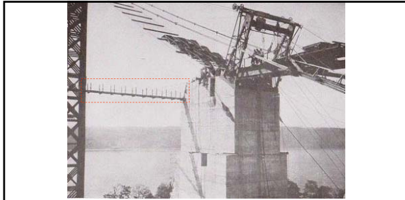
“...The floor beams, trusses and platforms for the side spans of the foot bridge, were assembled on pairs of low level ropes, and the floor beams are suspended from the groups of footbridge cable ropes above. The trusses and floors were erected from light platforms carried under 4-wheel carriages running on temporary ropes above the footbridge cables...”
