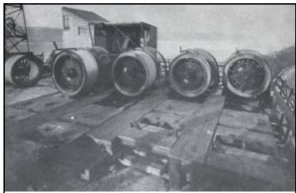
Above: caption: "Reels of cable wire mounted on unreeling machines at New York anchorage. Low level cats for shifting full and empty reels in foreground." 324
