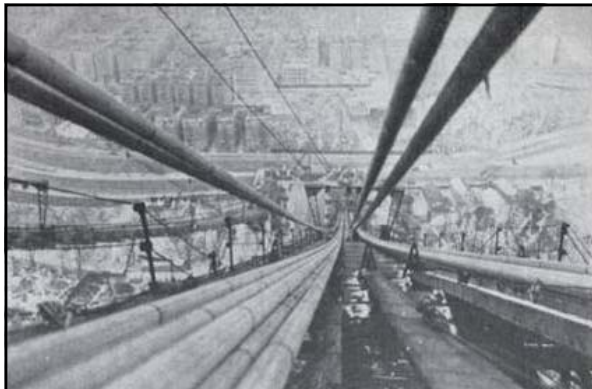
Above: caption: "Four strands completed and ready for adjustment with those already positioned in cable B" 341
