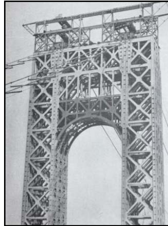
"...Integral with each construction tower is a transverse runway 245 feet long, cantilevering 21 feet beyond the north and south faces of the main tower for the 35 1/2 foot span girder crane, with two electrically operated pairs of 65-ton fixed hoists for lifting the cable strands. A 7 1/2-ton auxiliary hoist is also installed on each crane to operate whip lines or tackles on its cantilever extremities..."
