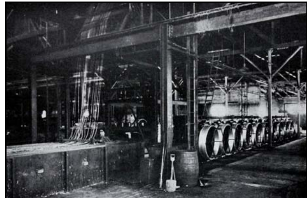
Above: caption: "Simultaneous galvanizing of twenty Hudson River Bridge cable wires, passing continuously and uninterruptedly through the zinc bath which deposits on them a coating of solid zinc from 1/1000 to 2/1000-inch in thickness." 244
