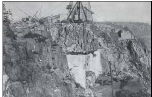
Above: caption: "Upper end of hoisting cableway on New Jersey shore, derrick mounted alongside of approach cut, commanding anchor block in cut" 256
