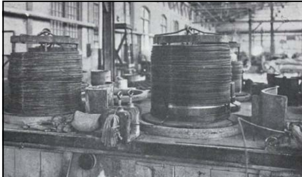
Above: caption: "Drawing bridge wire at the Kinkora plant, Roebing, N.J. (this wire drawing shop has a capacity of 5,000,000 pounds per month of bridge cable wire, and is producing 2,500,000 pounds per month to keep pace with the spinning of the Hudson River Bridge cables, and maintain an adequate reserve supply for them)." 241
