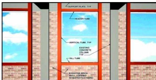
“...This solution has a tubular frame for each windowed wall panel, consisting of two vertical tubes horizontally braced with tubes welded at each window’s head and sill. The frame becomes the structural support for the blast-resistant windows, with the vertical tubes giving new blast protection to the infill walls...” STRUCTURE magazine, July/August 2001 Above: caption: “This illustration shows reinforcements added to the Pentagon’s walls as seen from the inside. Reinforced concrete columns are shown in gray, and tubular steel reinforcements are pictured in red.” 167
