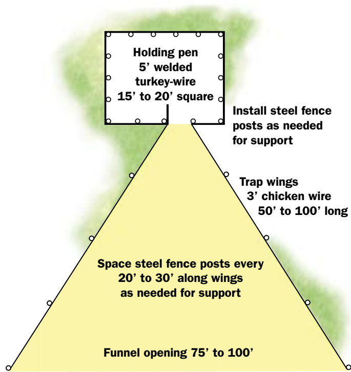
Figure 6-15. Canada goose funnel trap.
