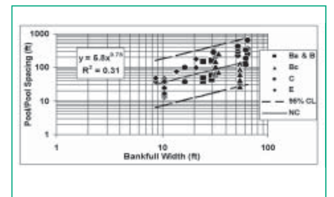
Figure 6.8 Pool-to-pool spacing as a function of bankfull width Clinton et al., 1999
