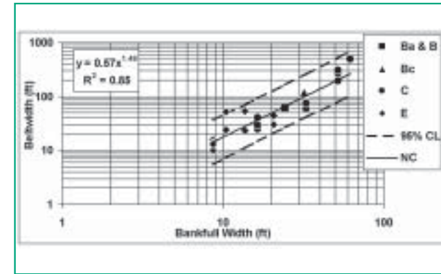
Figure 6.5 Belt width as a function of bankfull width Clinton et al., 1999
