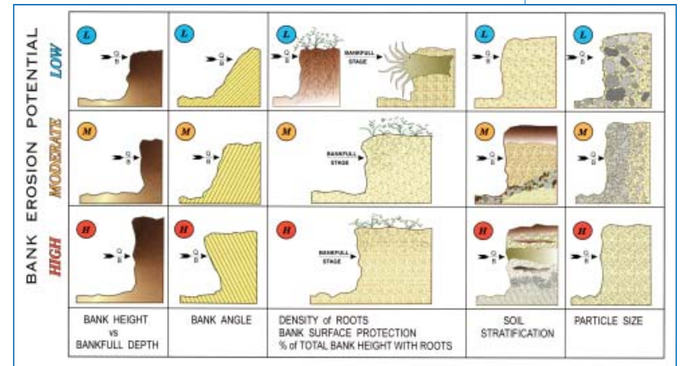
Fig. 3.9 Streambank erodibility factors Rosgen 1996, 6-40
