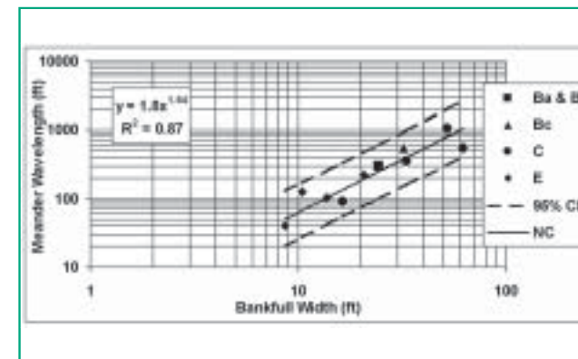
Figure 6.7 Meander wavelength as a function of bankfull width Clinton et al., 1999
