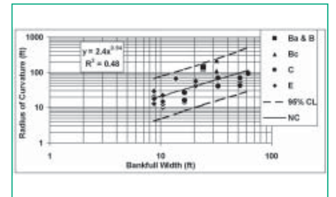
Figure 6.6 Radius of curvature as a function of bankfull width Clinton et al., 1999
