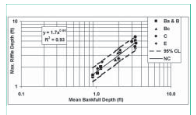
Figure 6.10 Max riffle depth as a function of mean bankfull depth Clinton et al., 1999
