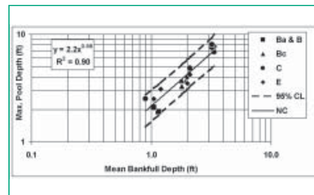
Figure 6.9 Max pool depth as a function of riffle mean bankfull depth Clinton et al., 1999
