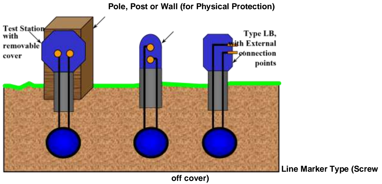
Figure 31 Abovegrade Test Station Pole, Post or Wall (for Physical Protection) Line Marker Type (Screw off cover)
