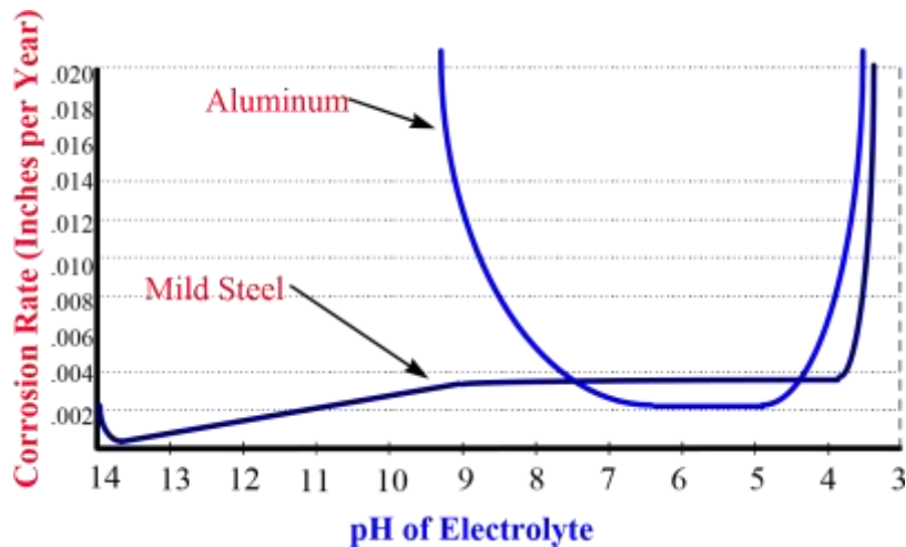
Figure 17 Effect of Electrolyte pH on the Rate of Corrosion
