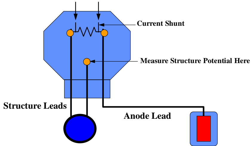
Figure 23 Potential - Current Test Station Connections
