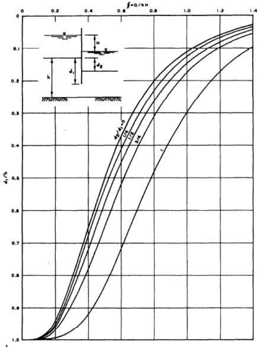
Figure 9 Flow beneath a partially penetrating cutoff wall.
