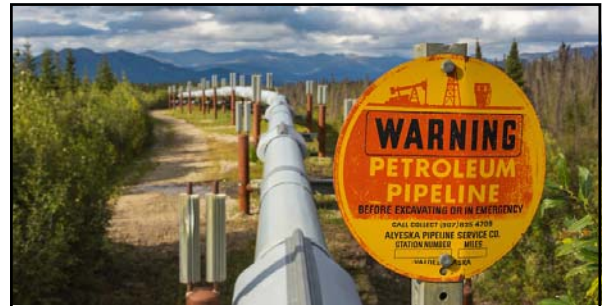
“...Of more immediate concern is the daunting task of repairing the corrosion. While the 48-inch-diameter pipeline runs aboveground on trestles for about half its length, virtually all of the corroded sections are buried in unstable permafrost. Thus, patching corroded areas necessitates not only welding on new steel jackets, but also excavating and reburying the pipe. The work will take years, and the cost will be staggering. Estimates range from $600 million to $1.5 billion. To date, only a fraction of the suspected corrosion spots has been repaired...” 890 Popular Mechanic, August 1990
