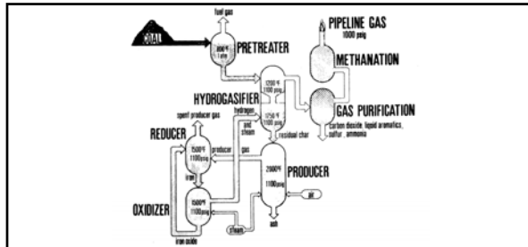
Above: caption: "Flow diagram of the steam-iron process integrated with the HyGas process." The steam-iron system comprises three principal vessels: 1) the producer, in which residual HyGas char is converted to reducing gases; 2) the reducer, in which iron oxide is reduced with producer gas, and; 3) the oxidizer, in which the iron is re-oxidized and the hydrogen is produced. In integrated operation, spent char from the HyGas process is fed directly to a producer vessel in which it reacts with air and steam to generate a gas capable of reducing iron oxide to iron. In actual operation, the producer zone is contained within the hydrogasifier pressure shell. 85
