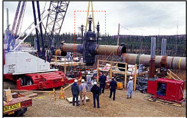
Above: caption: "A main line valve (RGV 80) is lifted from its site at MP 519 near Delta Junction, south of the midway point on the Trans-Alaska Pipeline, to be analyzed for sealing problems. Another valve from the Alyeska inventory replaced it in a 29-hour operation that shutdown the pipeline at the end of September 1998." 164
