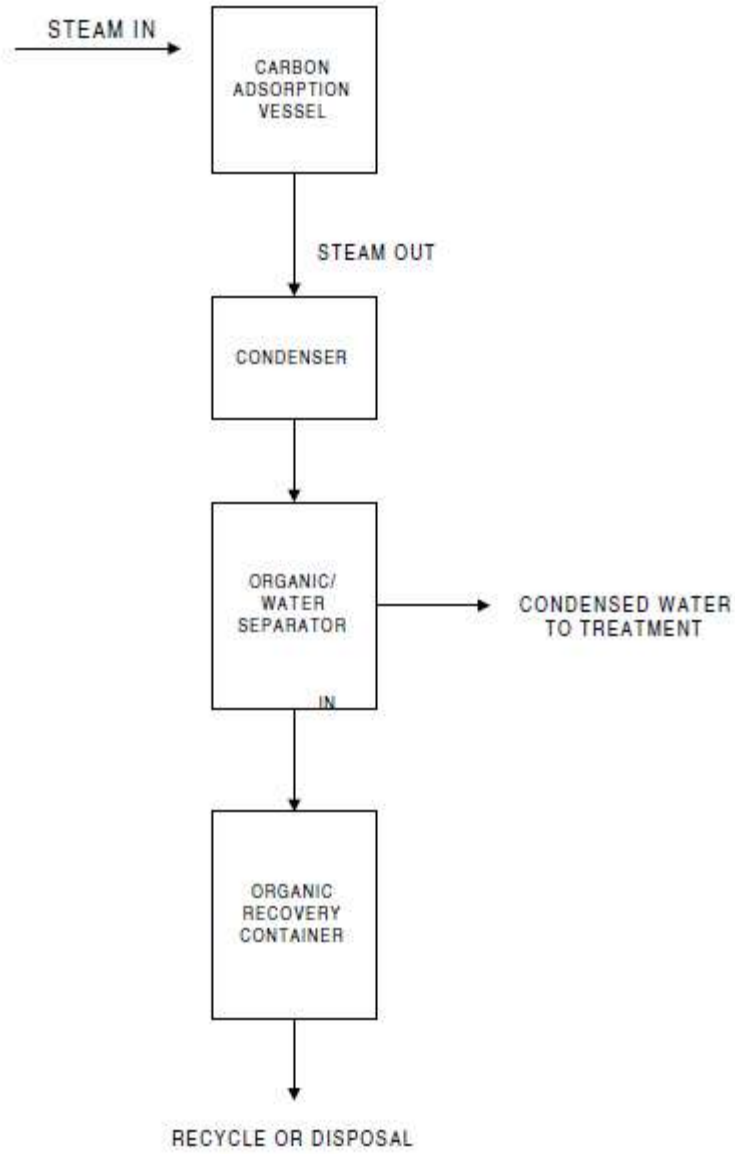
Figure 3-3 Steam regeneration.
