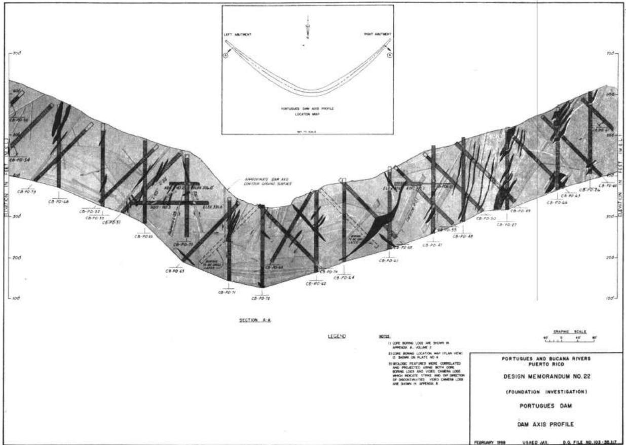
Figure 10-2 Arch dam boring profile from Portugues Dam Design
