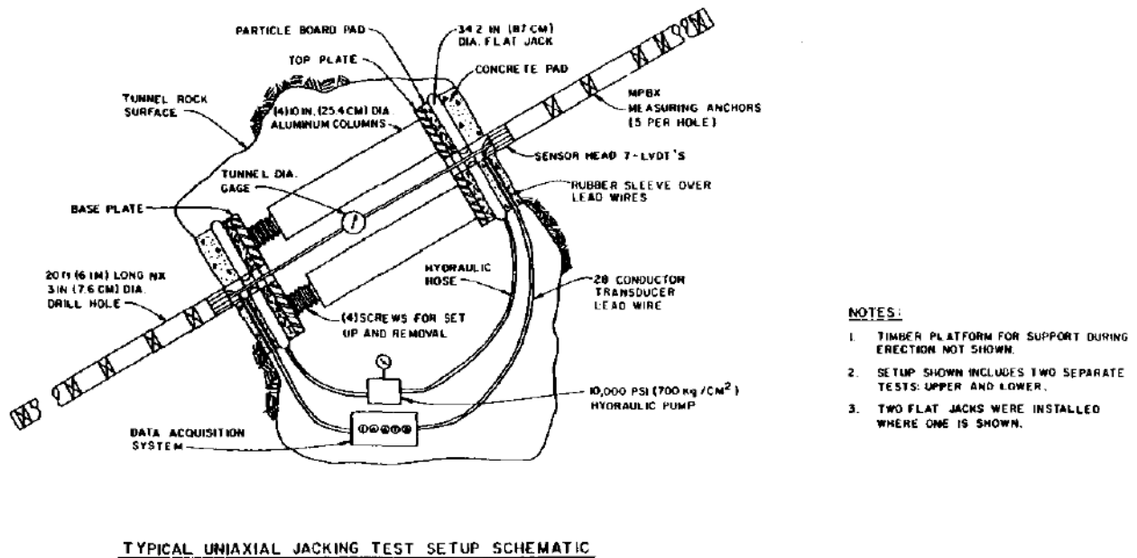
Figure 10-6 Uniaxial jacking test diagram from Portuges Dam
