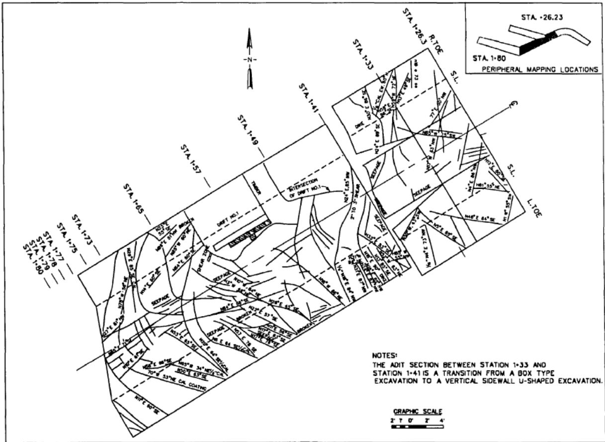
Figure 10-3 Adit periphery mapping plan view from Portugues Dam Design
