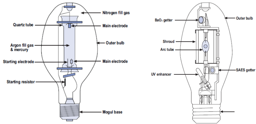
Figure 4 Construction of a high-pressure mercury vapor lamp and metal halide lamp
