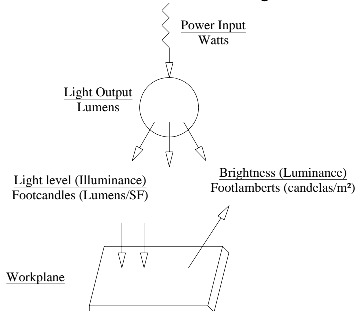
Figure 1 The concept of watt, lumens and illuminance
