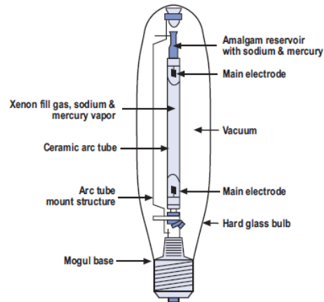
Figure 5 Construction of a high-pressure sodium lamp.
