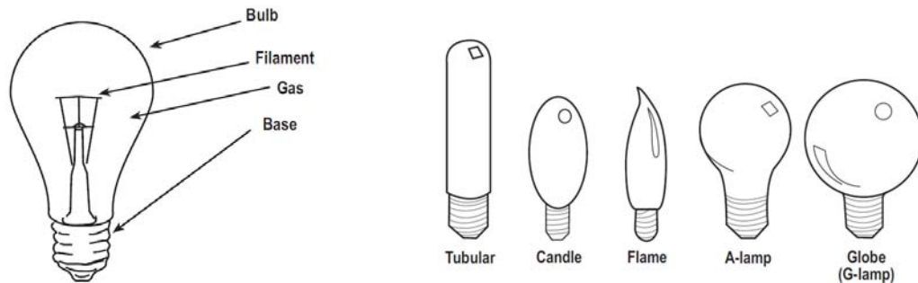
Figure 2 Construction of a typical incandescent lamp and common shapes
