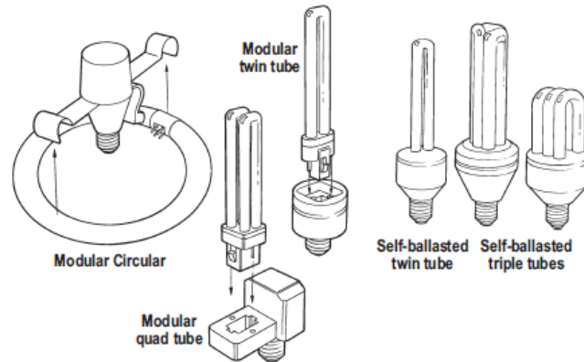
Figure 3 Different types of compact fluorescent lamps.
