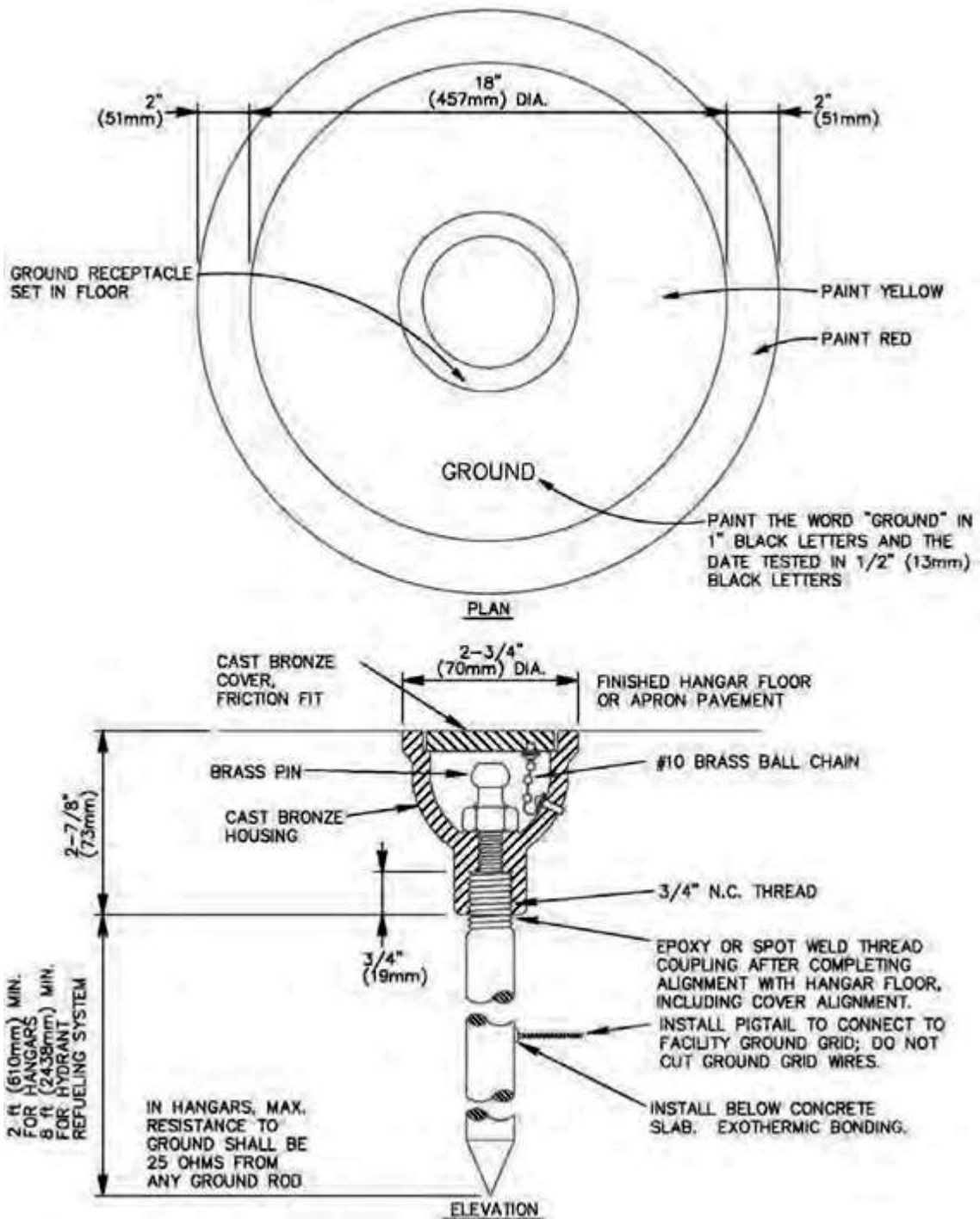
Figure 2.3 Grounding Receptacle.
