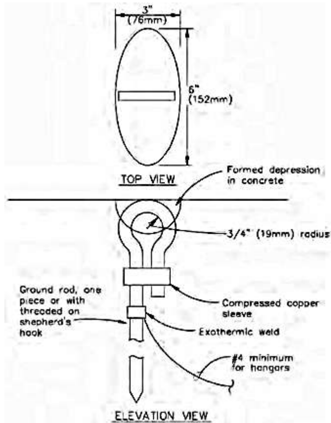
Figure 2.2 Static Grounding Point.
