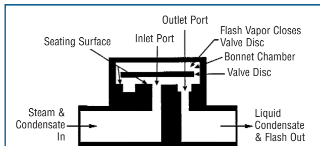
Figure 8. Thermodynamic Disc Steam Trap
