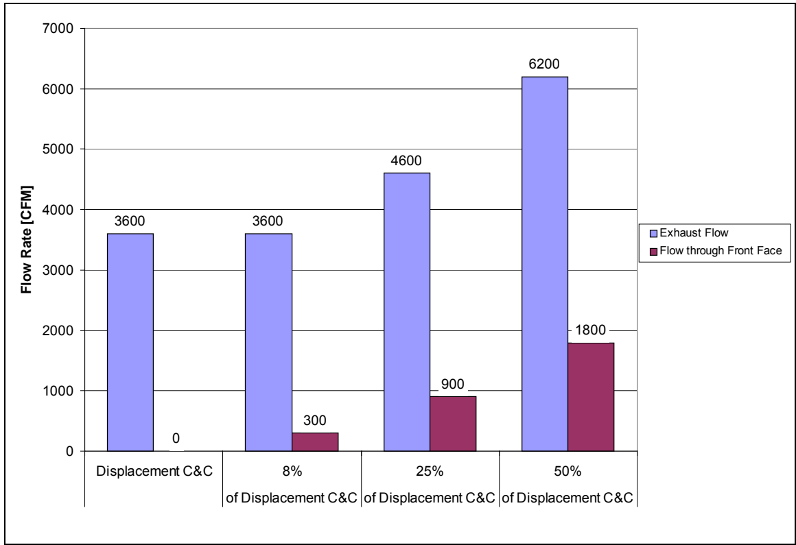
Figure 48: Exhaust and Front Face Airflow Rates as Front Face Airflow Rates were Increased as Percentages of the Original Displacement Ventilation Rate
