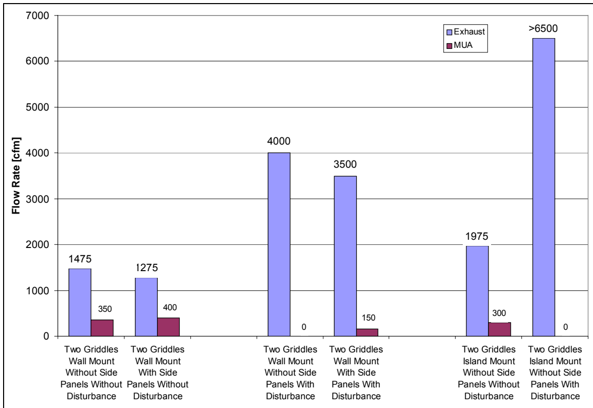
Figure 44: Exhaust and Front Face Flow Rates for the Two Griddles during Idle Conditions
