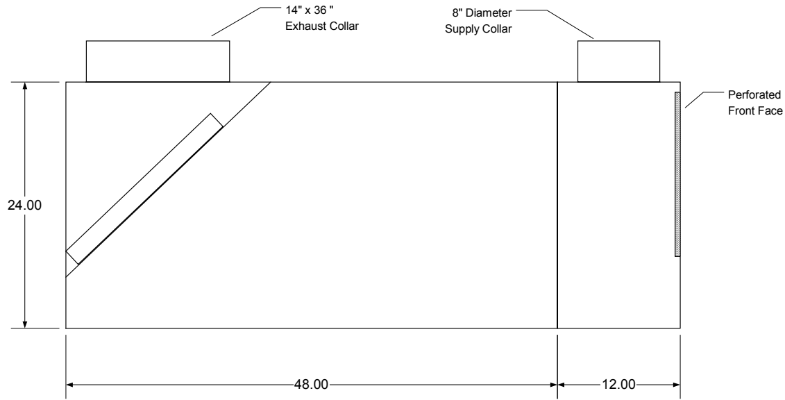
Figure 38: Cross-Section Drawing of Front Face Plenum and Canopy Hood
