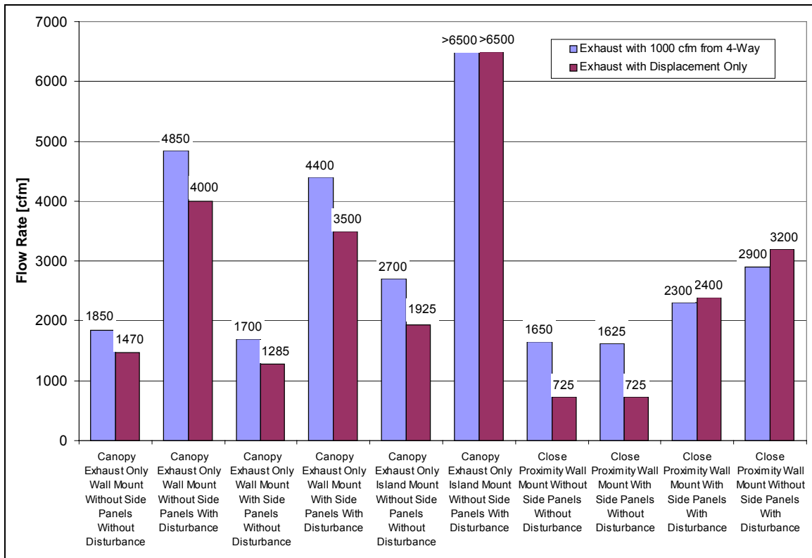
Figure 67: Exhaust Flow Rates for the Two Griddles During Idle Conditions Under Canopy and Proximity Hoods for Displacement and 1000 cfm through the Center Front 4-Way Diffuser
