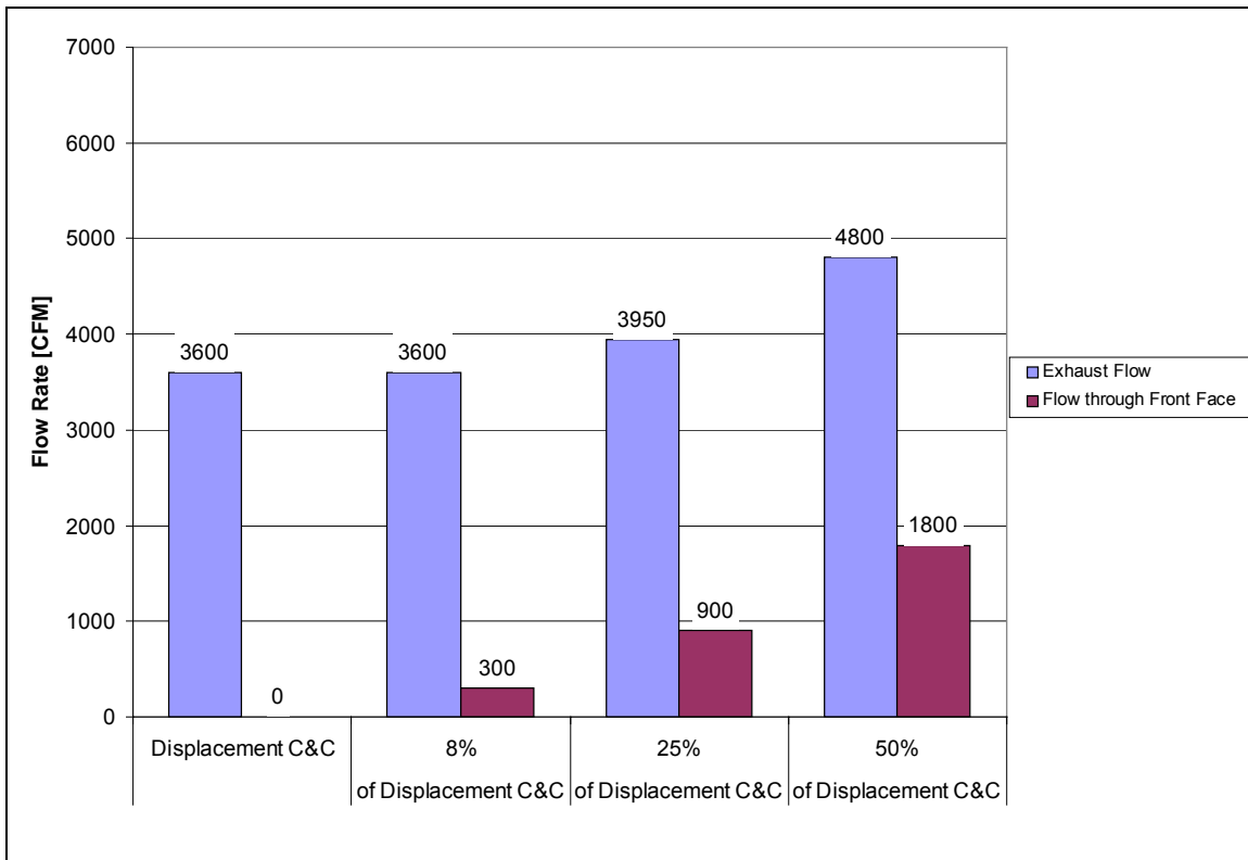
Figure 51: Exhaust and Front Face Airflow Rates as Front Face Airflow Rates were Increased as Percentages of the Original Displacement Ventilation Rate with Modified Supply Plenum
