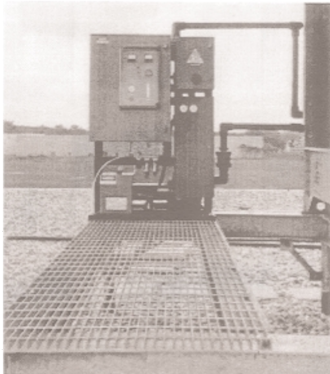
Fig. 1. Typical Cooling Tower Ozone Generation System
