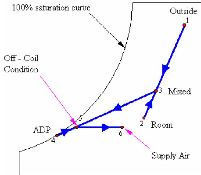
PSYCHROMETRIC CHART SHOWING TYPICAL SUMMER CYCLE
