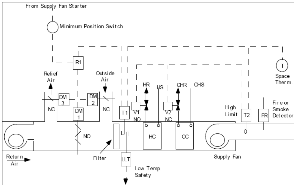
Single Zone - All Direct Control from Space Thermostat
