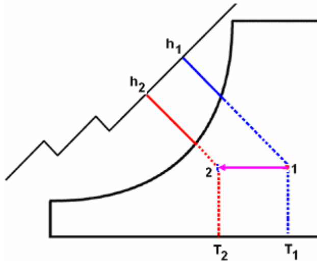
Sensible Cooling
