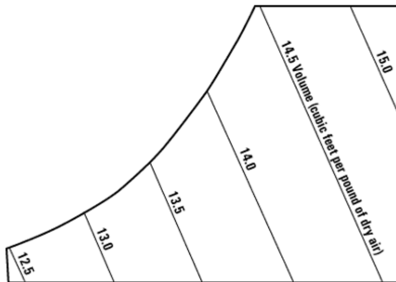
Specific Volume lines shown on Psychrometric Chart
