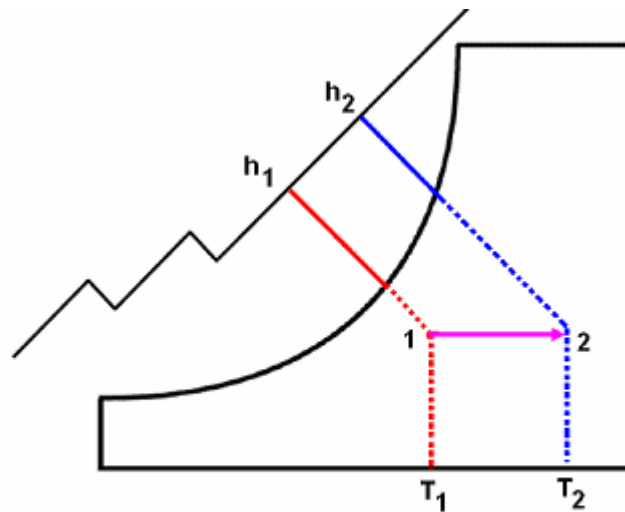
Sensible Heating
