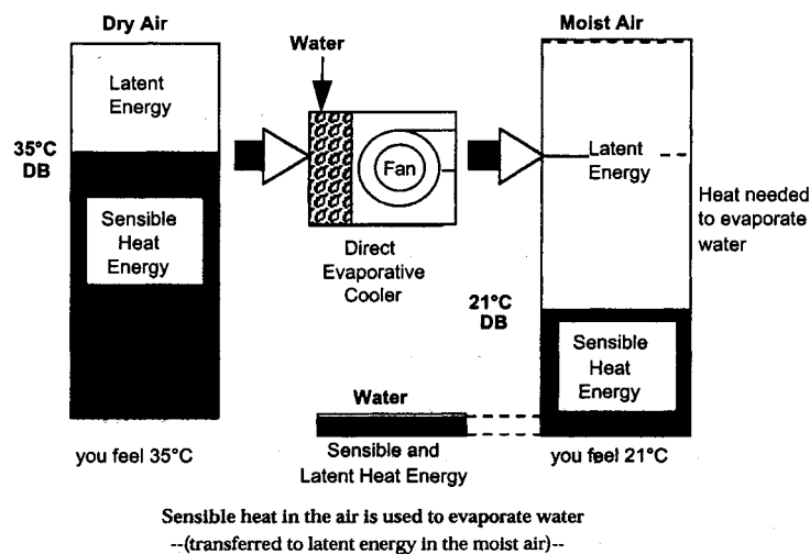
Figure 14: Simplified Evaporative Air-Conditioning Process 14
