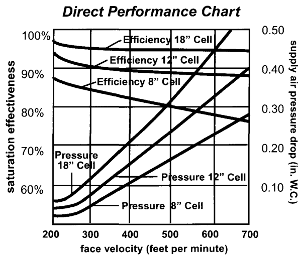
Figure 12: Direct EAC Effectiveness for Rigid Media 13
