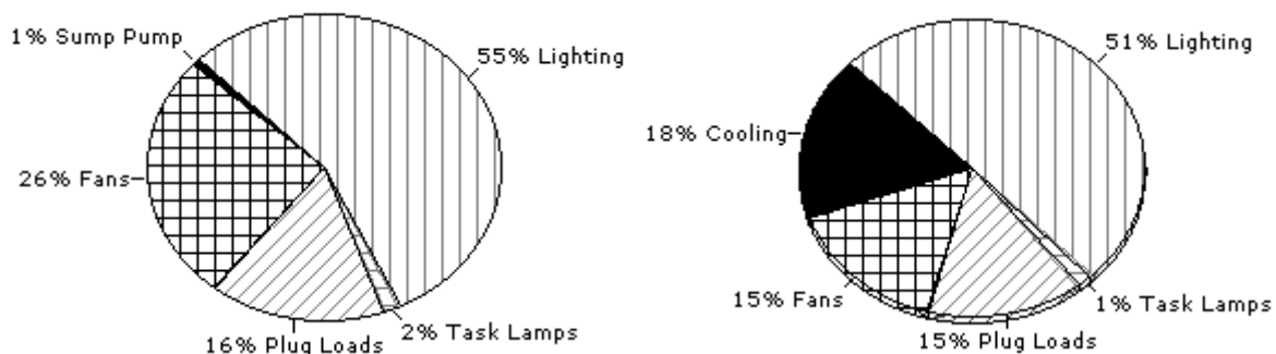
Figure 1: Comparative Electricity Annual Use for a Direct EAC and Refrigerated Air
