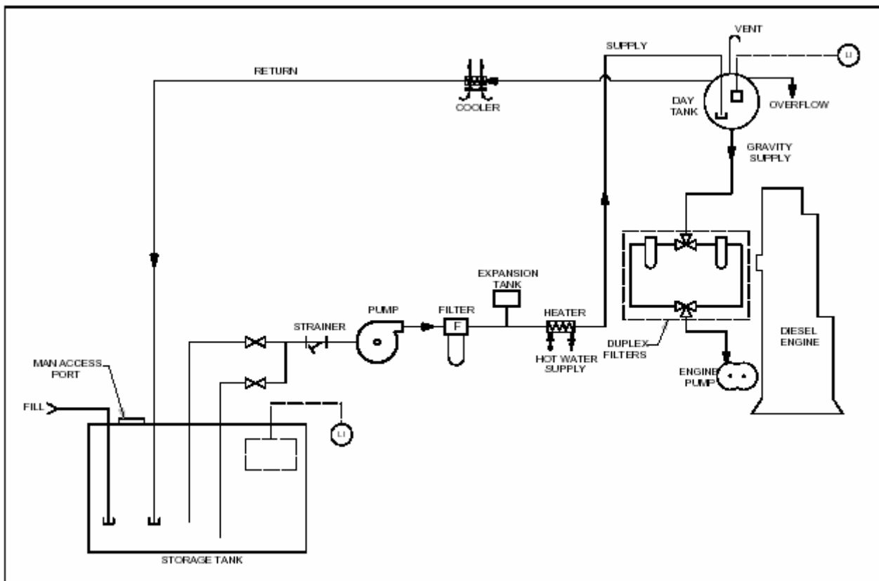
Figure 5-1 Schematic of a typical fuel system
