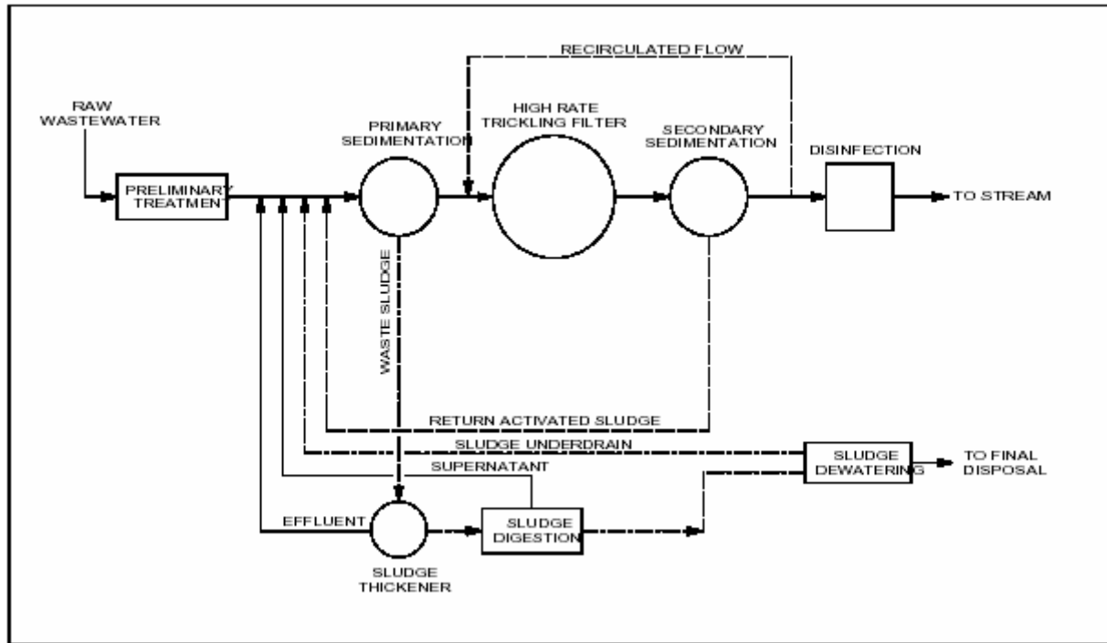
Figure 9-4 Sewage trickling Filter Process
