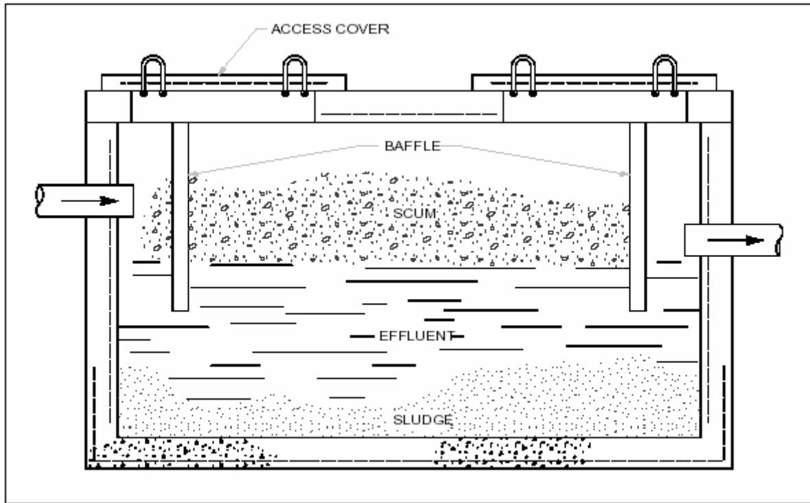
Figure 9-3 Cross Section of a Septic Tank
