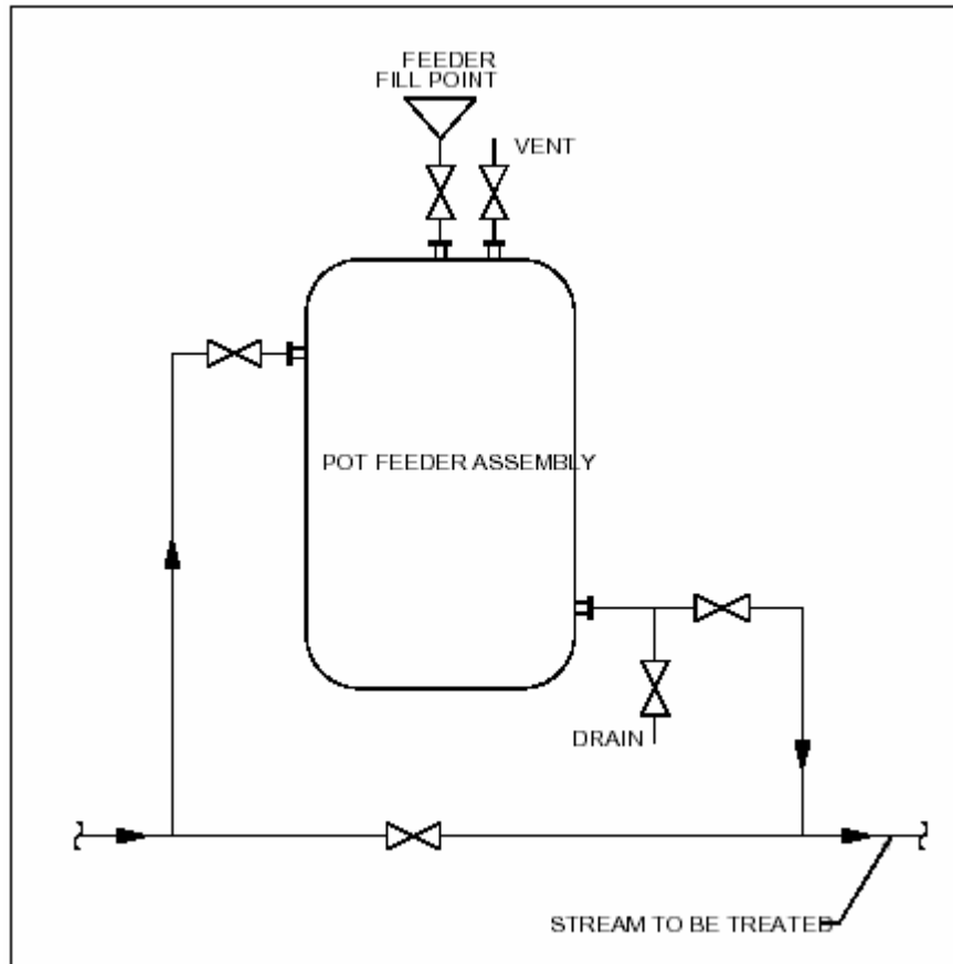
Figure 9-2 Schematic of a Process Water Treatment System
