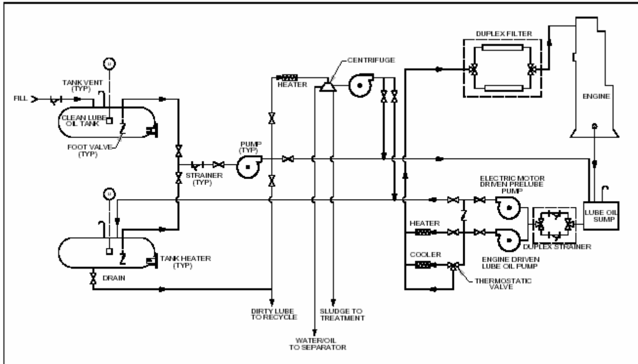
Figure 5-2 Schematic of a typical lube oil system
