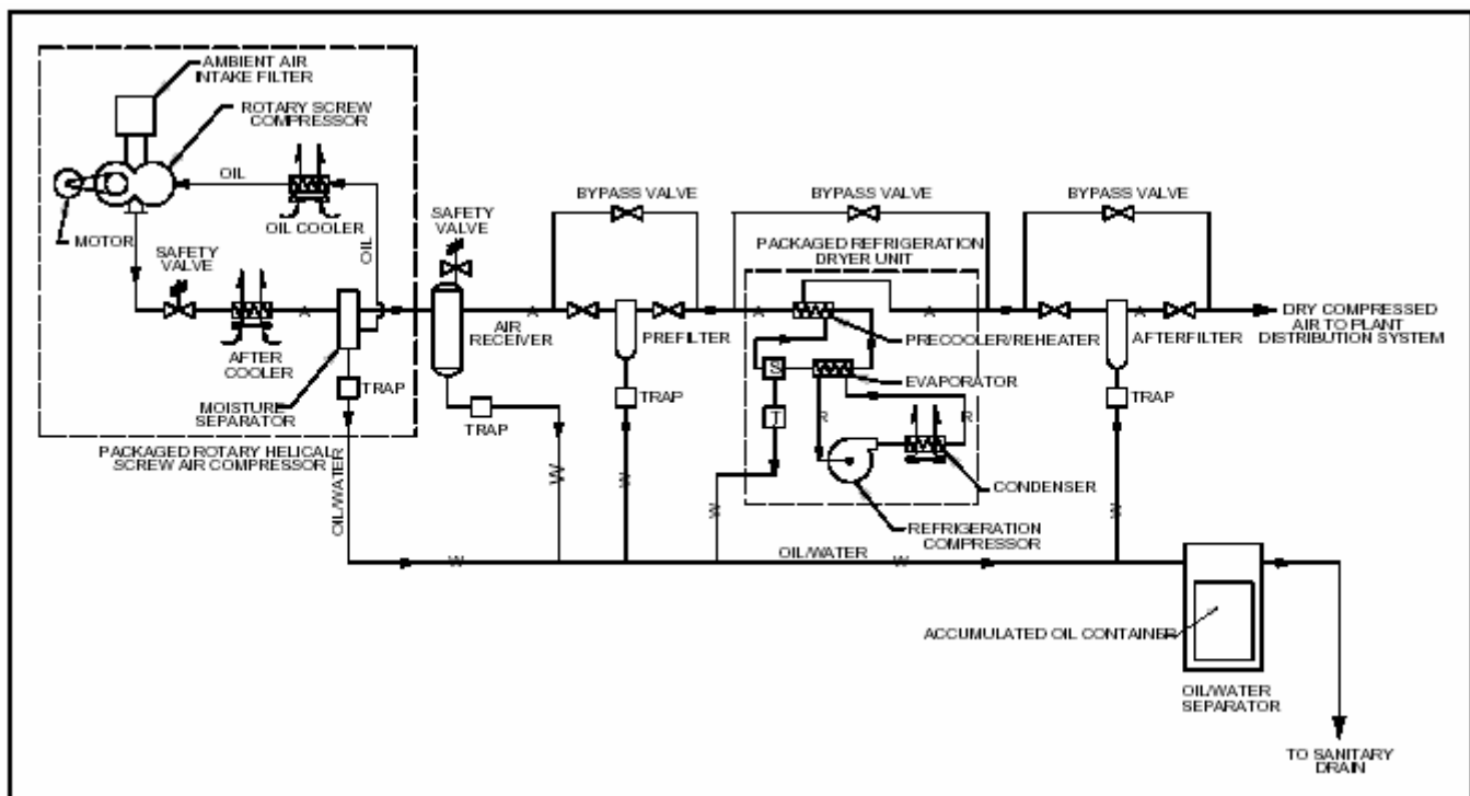
Figure 6-1 Schematic of a typical compressed air system
