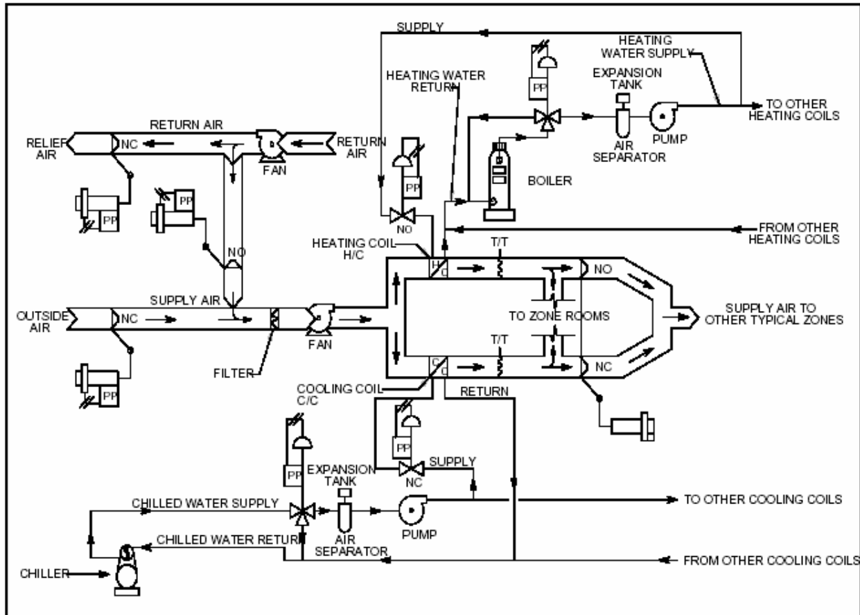
Figure 4-1. Schematic of a typical HVAC system
