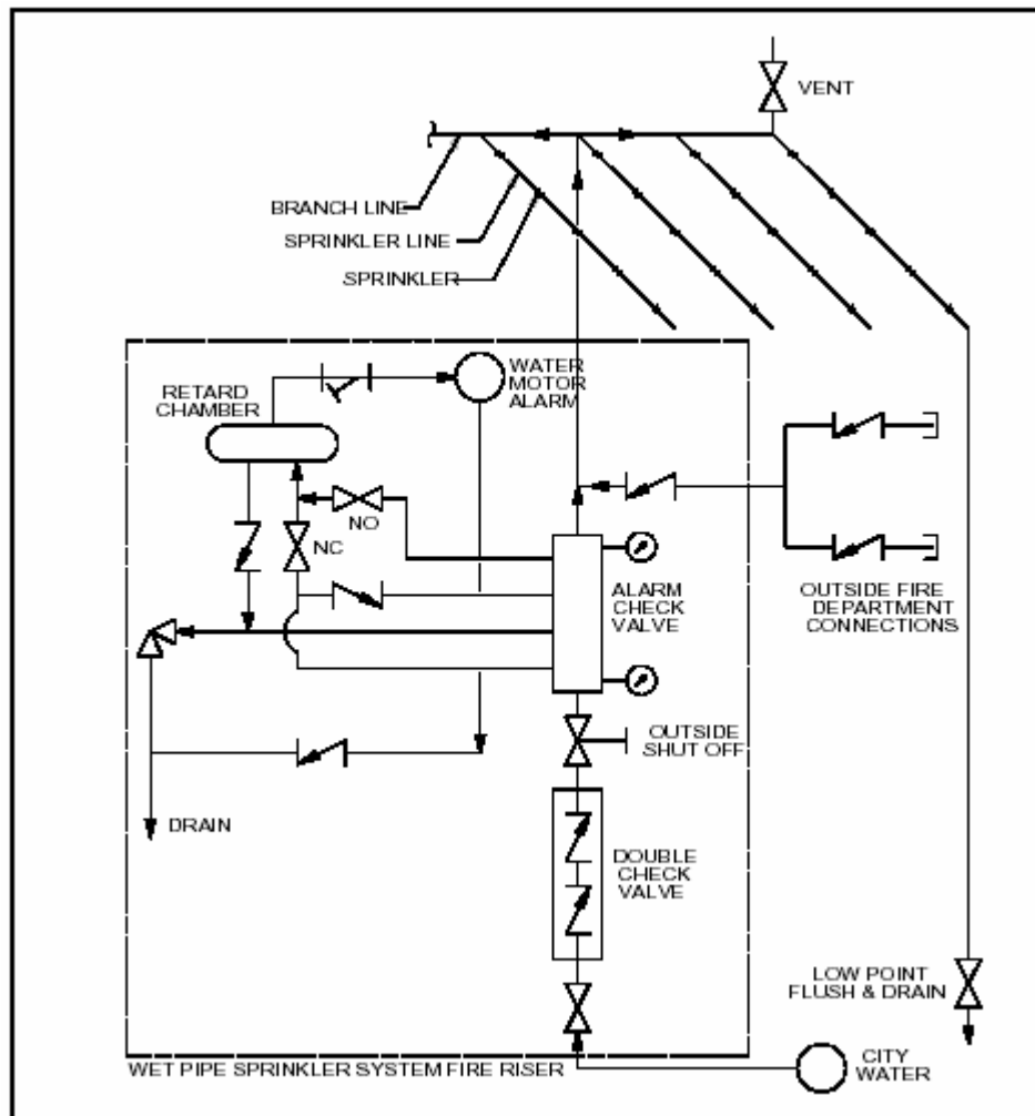
Figure 7-1 Typical Wet Pipe Sprinkler System
