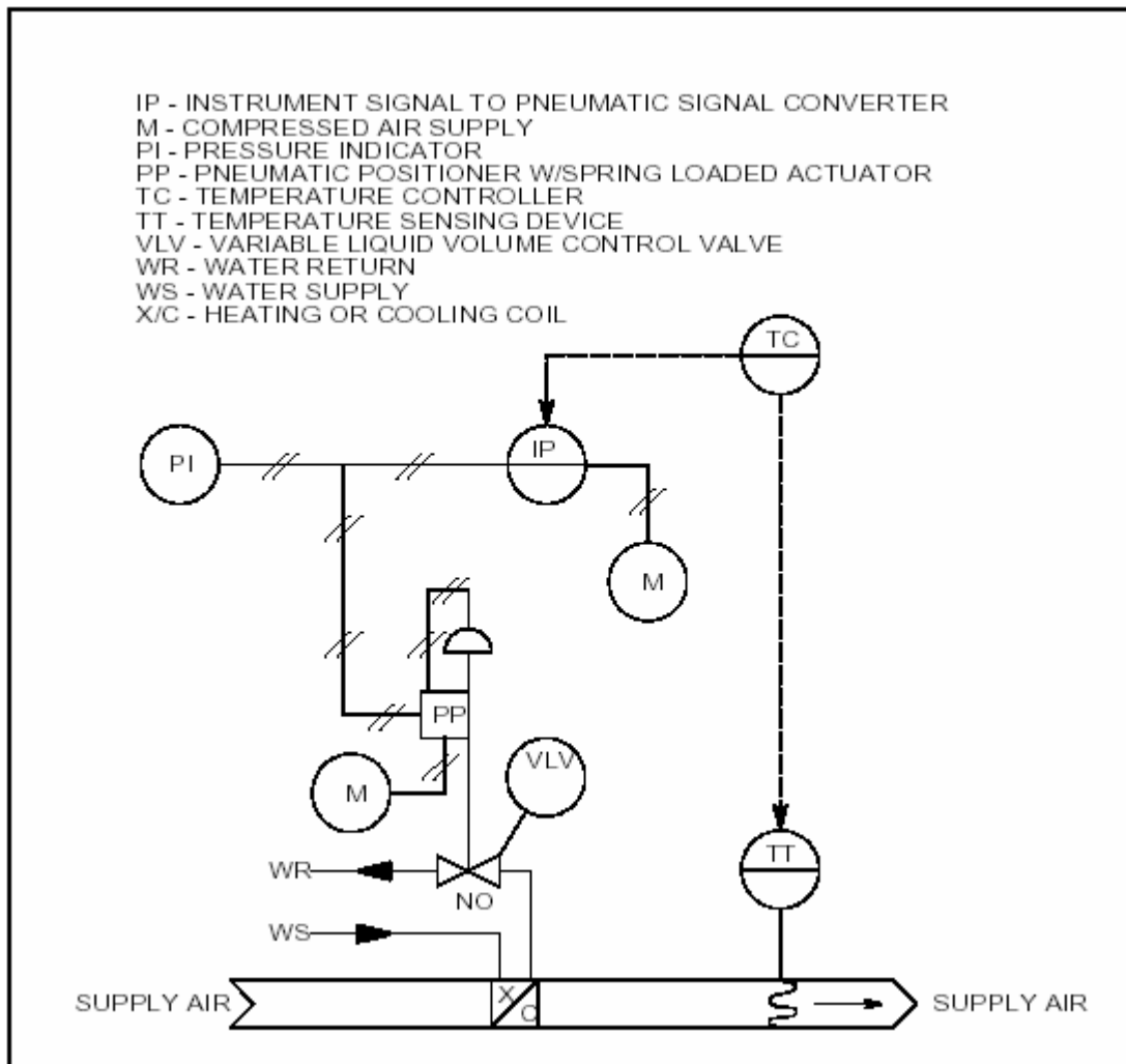
Figure 4-2. Typical HVAC control loop
