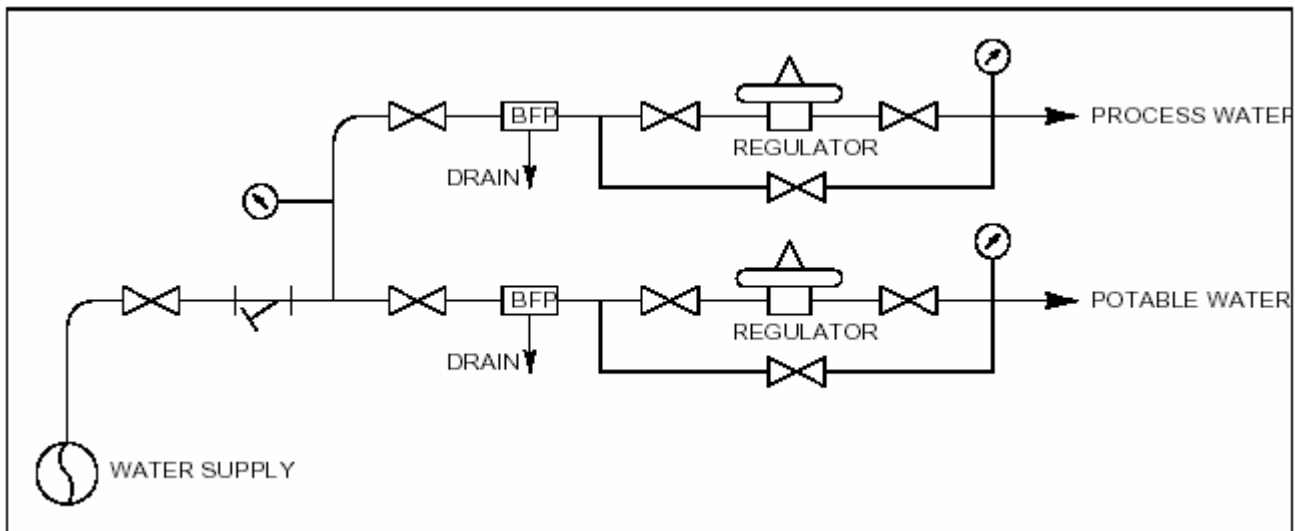
Figure 9-1 Schematic of a Typical Potable and Process Water System
