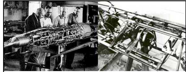
Left: caption: "Goddard Series P Rocket of large fuel capacity, with the rocket motor, pumps, and turbines in view"
