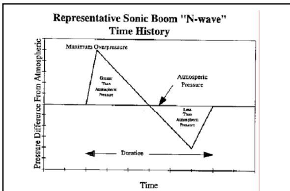
Above: caption: "Representative Time History of a Sonic Boom "N-wave" Pressure Pulse"
