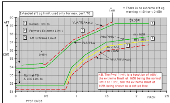
Above: Center of Gravity (CG) corridor diagram
