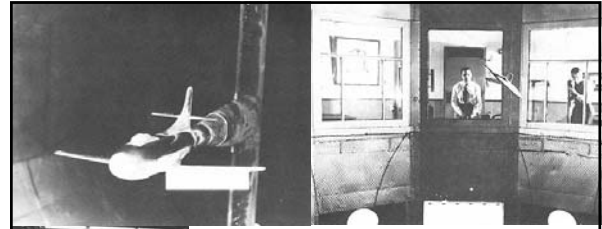
Above L&R: Models of the D-558 were tested in the 8-Foot High-Speed Tunnel (left) in June 1947 and in the 20-Foot Spin Tunnel (right) five months later
