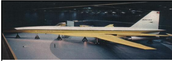
The Boeing variable-geometry SST dream was never realized. The variable-sweep wing idea was abandoned (due to excessive hinge weight) in October 1968 and the 2707-300 was cut to 234 seats with a fixed delta wing mounted ahead of a horizontal tail. It used essentially the same fuselage and engines as the preceding version. A full-size wooden mock-up and two prototypes were begun in September 1969. By this time, the project was already two years behind schedule and the Anglo-French Concorde had already made its first successful flight; on March 2 nd 1969. Amid growing public protests against Concorde , the U.S. Senate closed down the Boeing SST program completely on March 24 th 1971. Above: caption: "Side view of the Boeing 2707 full-size mockup" 235
