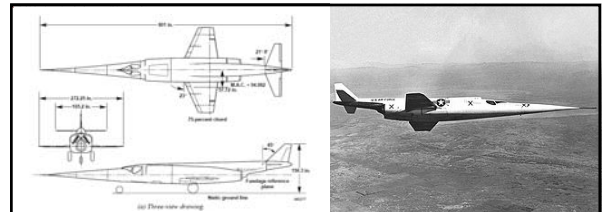
The Douglas X-3 "Stiletto" (above L&R) was an experimental jet aircraft with a slender fuselage and a long tapered nose. Its primary mission was to investigate the design features of an aircraft suitable for sustained supersonic speeds which included the first use of titanium in major airframe components. Douglas designed the X-3 with the goal of a maximum speed of approximately 2K mph, but it was seriously underpowered for this purpose and could not even exceed Mach 1 in level flight. Although the research aircraft was a disappointment, Lockheed designers used data from the X-3 tests for the Lockheed F-104 "Starfighter" which used a similar wing design in a successful Mach 2 fighter. The X-3 featured an unusual, rakish shape of a long cylindrical fuselage with tiny trapezoidal wings. The extended nose was to allow for the provision of test equipment. The X-3 50 first flew on October 15 th 1952.
