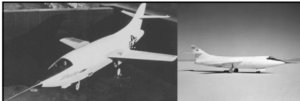
Above: the Douglas D-558-II "Skyrocket" (original flush canopy configuration, at left) was the follow up design to the Skystreak, with all the design work on the Skyrocket being done by the end of 1945, even before the D-558-1 had taken to the air (the D-558-1 fuselage could not be modified to accommodate both rocket and jet power). Powered by a Westinghouse J34-W-40 axial-flow turbojet engine with 3K-lbs. of thrust and a Reaction Motors XLR-8-RM-5 rocket engines making 6K-lbs. of thrust. The first flight was made on February 4 th 1948 (powered by the Westinghouse engine alone since the rocket motor was not ready in time). A number of changes were made after the first test flight/s including a new raised canopy (right) and larger tailfin. Also, the jet engine was removed to make way for more fuel for the rocket motor. The Skyrocket's flight research was done at the NACA's Muroc Flight Test Unit, re-designated the "High-Speed Flight Research Station" (HSFRS) in 1949. The HSFRS became the "High-Speed Flight Station" in 1954 and is now known as the "NASA Dryden Flight Research Center." The three aircraft produced gathered a great deal of data about pitch-up and the coupling of lateral (yaw) and longitudinal (pitch) motions; wing and tail loads, lift, drag and buffeting characteristics of swept-wing aircraft at trans-sonic and supersonic speeds and the effects of the rocket exhaust plume on lateral dynamic stability throughout the speed range. Information about the effects of external stores (bomb shapes, drop tanks etc.) upon the aircraft's behavior in the trans-sonic region (roughly 0.7 to 1.3 times the speed of sound) was also gained.
