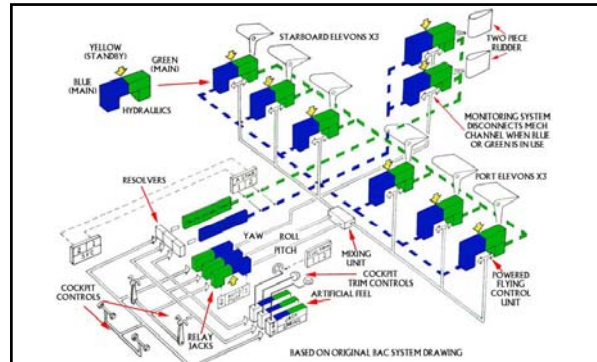
Above: caption: “Concorde was one of the first fly-by-wire aircraft in the world. With fly-by-wire, the aircraft is controlled by means of electrical signals that are sent to the hydraulically actuated flight controls.”
