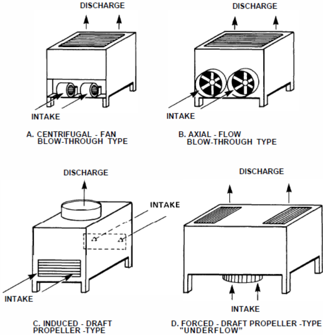
Figure 3 Principal types of cooling towers
