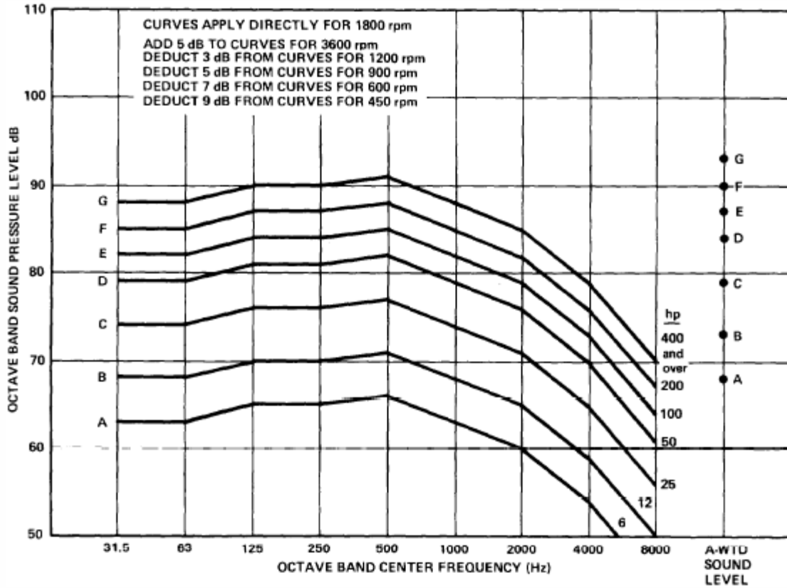
Figure 7 Sound Pressure Levels of DRPR Motors at 3 ft. Distance.
