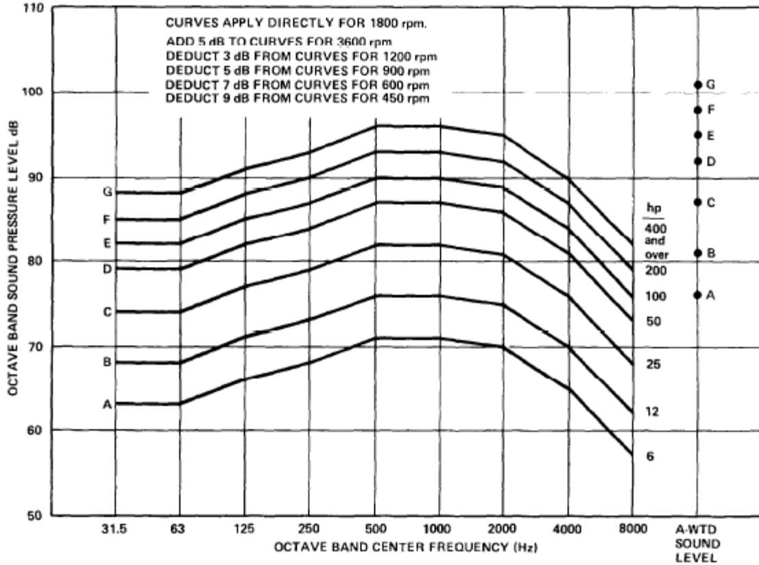
Figure 6 Sound pressure levels of TEFC motors at 3-ft. distance.
