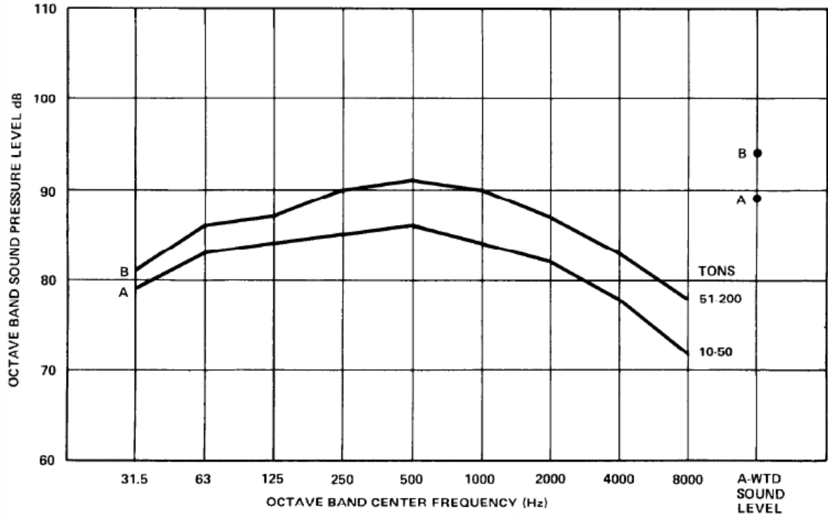
Figure 1 Sound pressure levels of reciprocating compressors at 3-ft. distance
