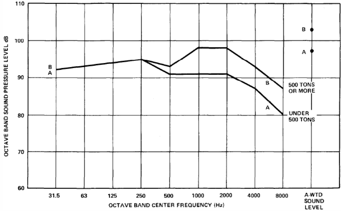
Figure 2 Sound pressure levels of centrifugal compressors at 3-ft. distance
