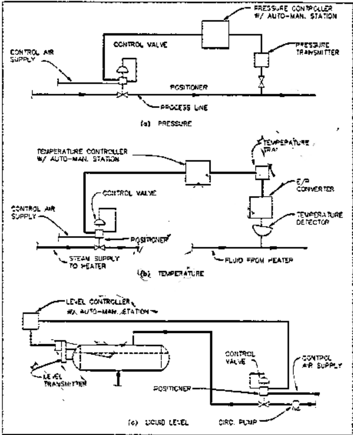
Figure 2 Typical control loops
