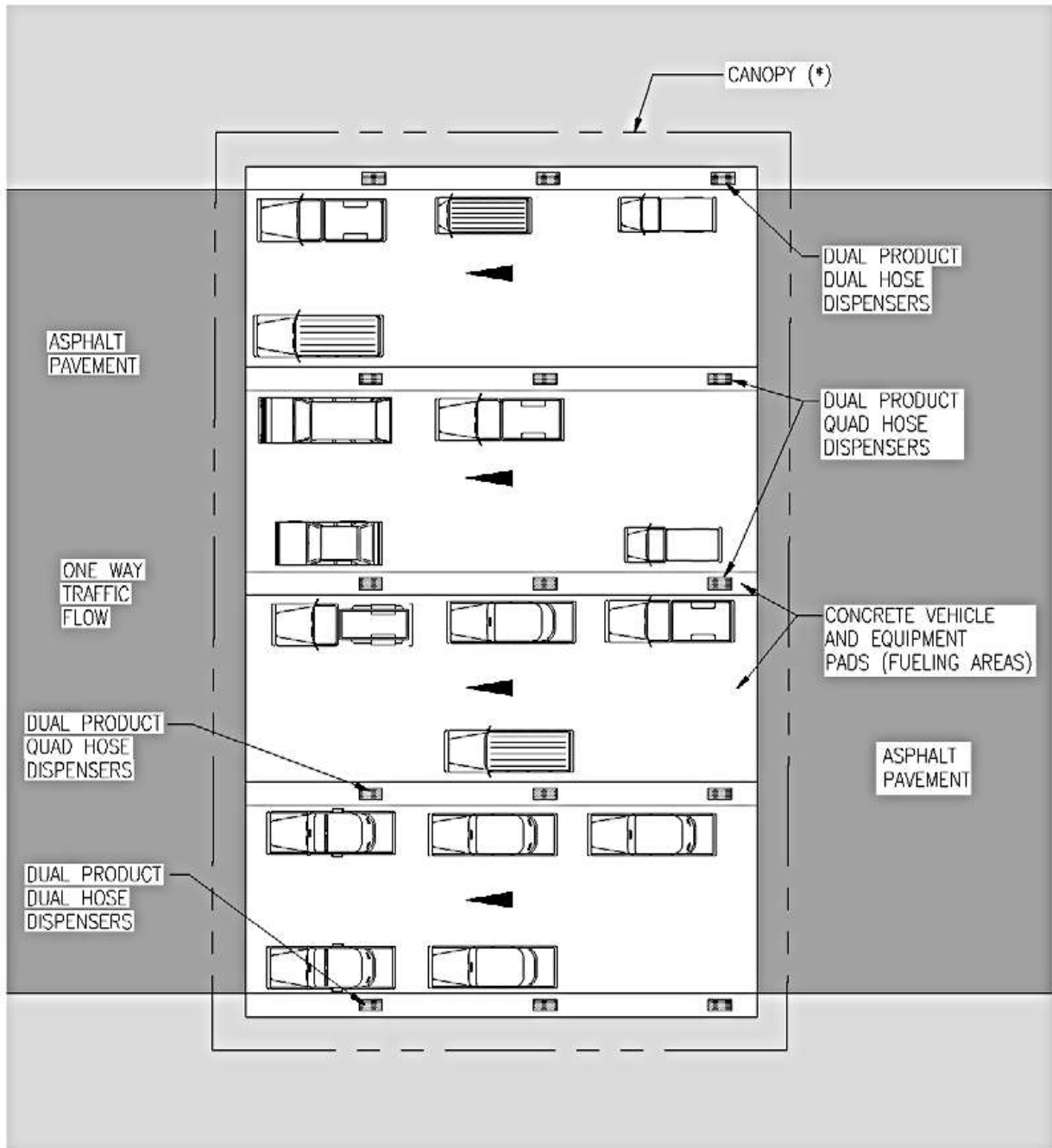
Figure 5 Vehicle Motive Fuel Filling Station Plan
