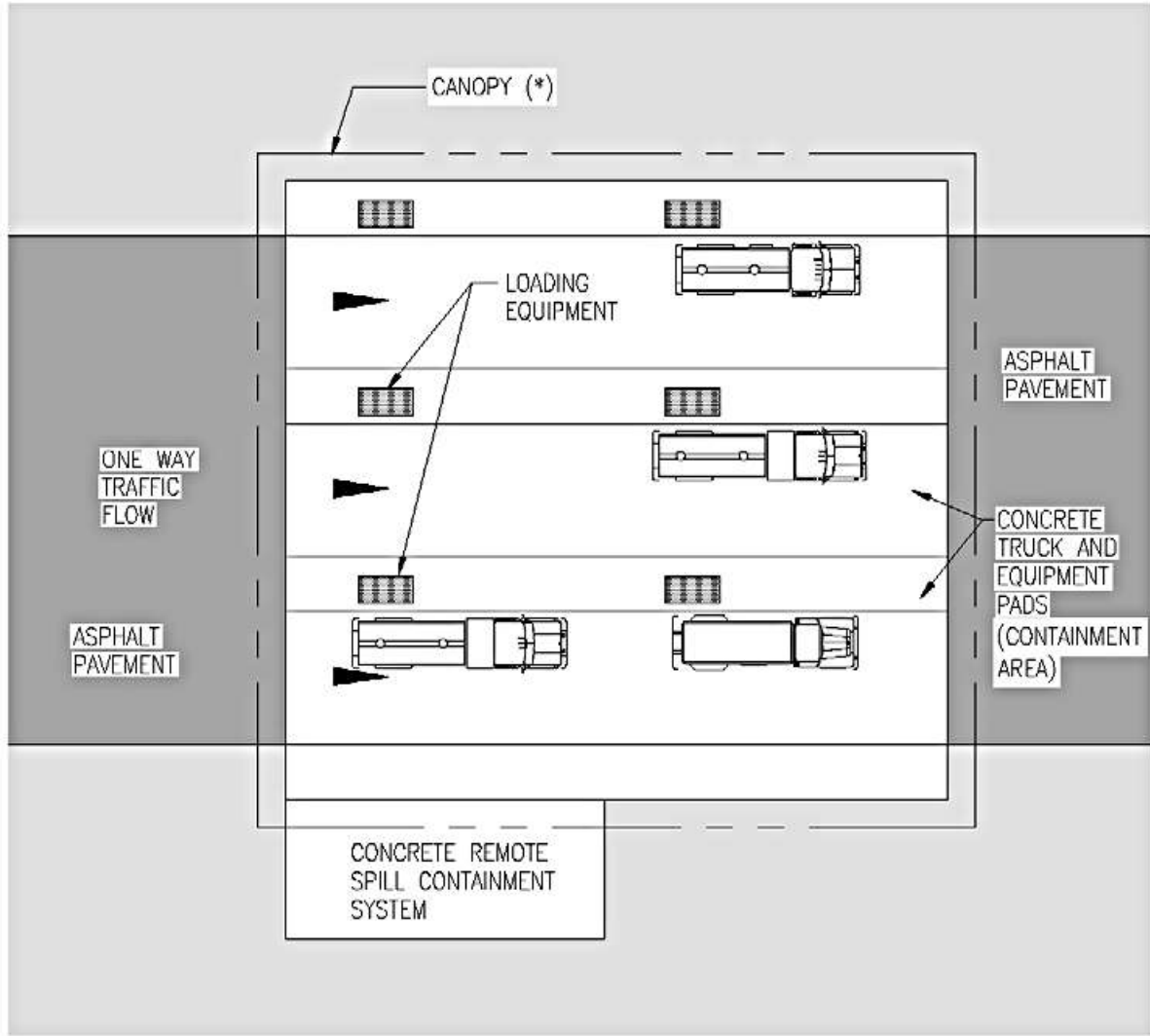
Figure 6 Refueler Ground Product Truck Loading Facility Plan
