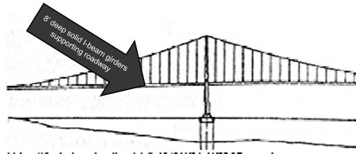
Moisseiff's design, elevation detail, 1940 WSA, WSDOT records
