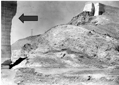
St. Francis Dam, Former West Abutment (Attribution: U.S. Geological Survey Photographic Library)
